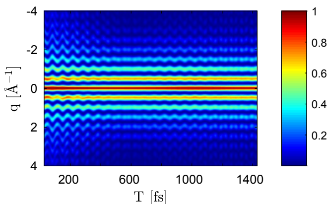
Fig. 6. Two-molecule contribution for NaF according to Eq. 18: Momentum transfer vs. probe delay with a temporal width of the probe pulse of 2.5 fs (FWHM). The intensity of the pattern is normalized.
