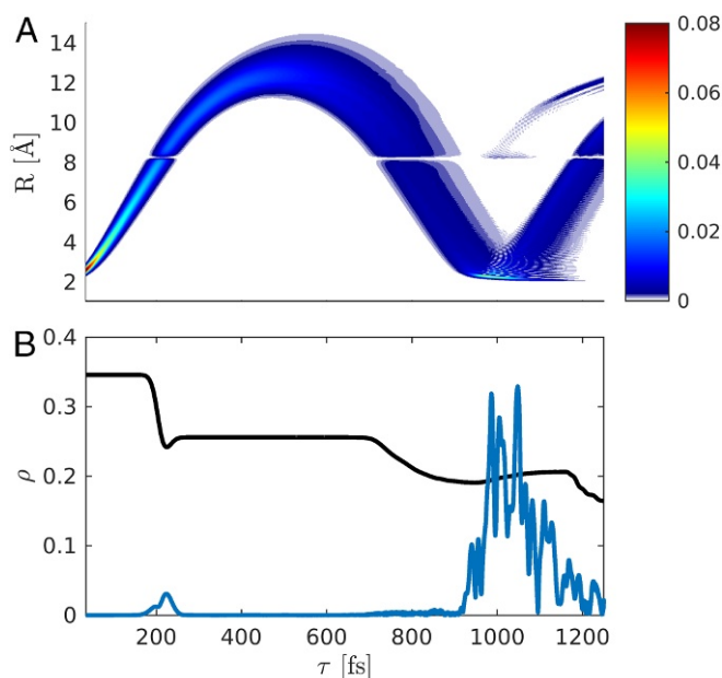
Fig. 3. Time evolution of the nuclear wave packet in the in the covalent A^1\Sigma state following excitation with a 10-fs pump-pulse (FWHM). (A) Probability density. (B) Excited-state population ( A^1\Sigma , black) and the magnitude of the coherence |\tilde{\rho}_{eg}| (blue). The initial coherence created by the pump pulse ( T < 50 fs) is not shown.
