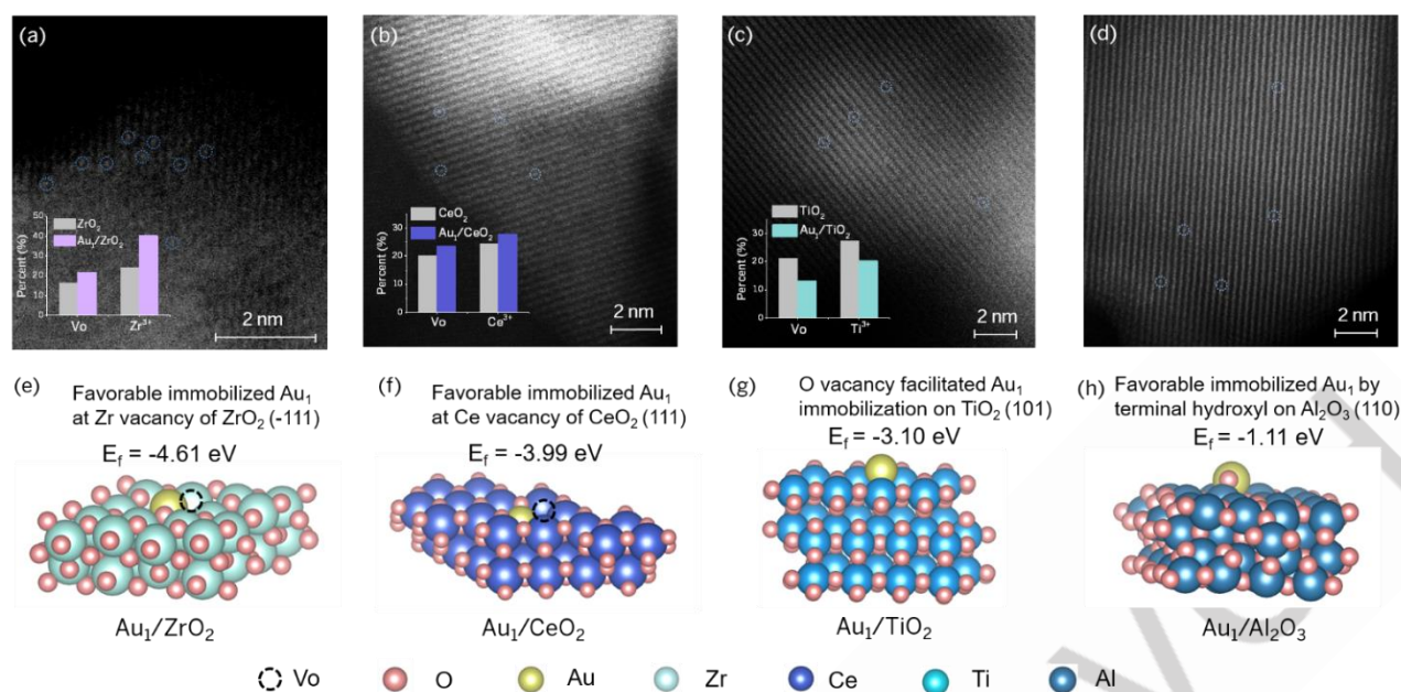
Figure 1. The optimized structure of four ADC prototypes. AC-HAADF-STEM images for (a) Au 1 /ZrO 2 , (b) Au 1 /CeO 2 , (c) Au 1 /TiO 2 and (d) Au 1 /Al 2 O 3 . Atomically dispersed Au atoms are highlighted by blue circles. The insets in Figure 1a-1c show the percent evolution of oxygen vacancy (Vo) and coordinatively unsaturated metal ions (Zr 3+ , Ce 3+ , Ti 3+ ) for the catalysts before and after Au atom insertion based on XPS deconvolution (Figure S5-S7); DFT models of Au atom on various oxide supports: (e) Zr vacancy immobilized Au 1 on ZrO 2 (-111), (f) Ce vacancy immobilized Au 1 on CeO 2 (111), (g) Vo immobilized Au 1 on TiO 2 (101), and (h) Terminal hydroxyl stabilized Au 1 on Al 2 O 3 (110).
