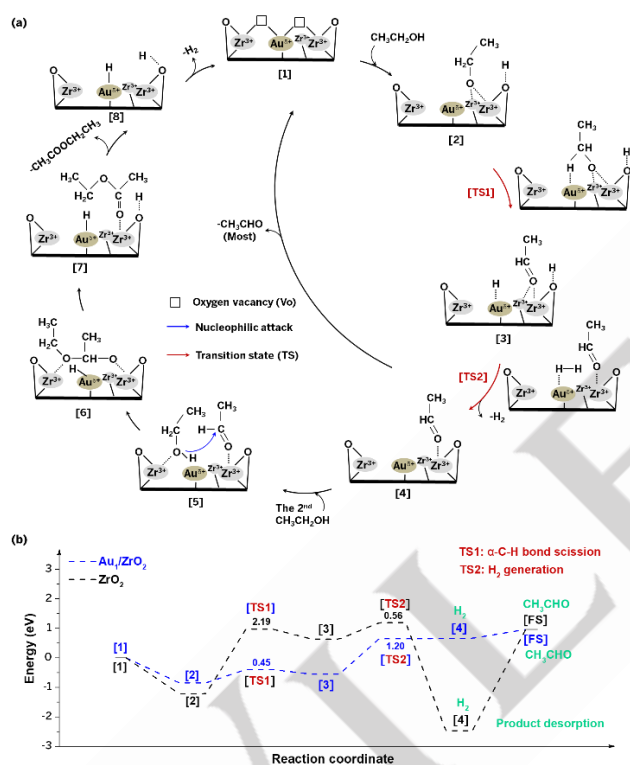
Figure 4. Zr^{3+} -Vo- Au^{\delta+} complex site-mediated ethanol dehydrogenation on Au_1/ZrO_2 . (a) Catalytic cycle simulations of ethanol dehydrogenation on Au_1/ZrO_2 . (b) The calculated energy profiles of ethanol dehydrogenation to acetaldehyde on Au_1/ZrO_2 and ZrO_2 .
