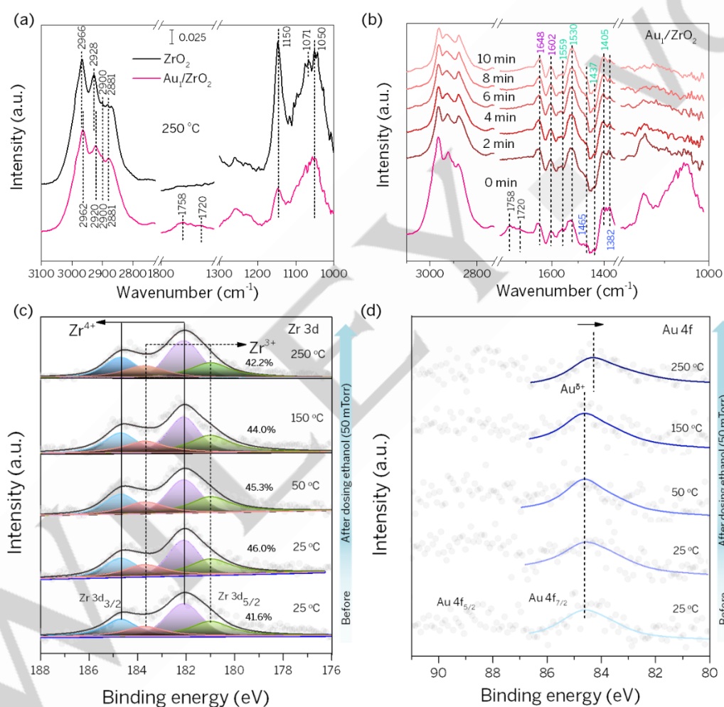
Figure 3. Spectroscopic studies on ethanol dehydrogenation over \text{Au}_1/\text{ZrO}_2 . (a) In-situ diffuse reflectance infrared Fourier transform spectra (DRIFTS) of \text{Au}_1/\text{ZrO}_2 and \text{ZrO}_2 when purging with ethanol vapor (with \text{N}_2 as carrier gas) at 250 °C; (b) Time-resolved in-situ DRIFTS of \text{Au}_1/\text{ZrO}_2 purged with pure \text{N}_2 (without ethanol vapor dosing); In-situ AP-XPS (c) Zr 3d and (d) Au 4f spectra for \text{Au}_1/\text{ZrO}_2 before and after ethanol dosing.
