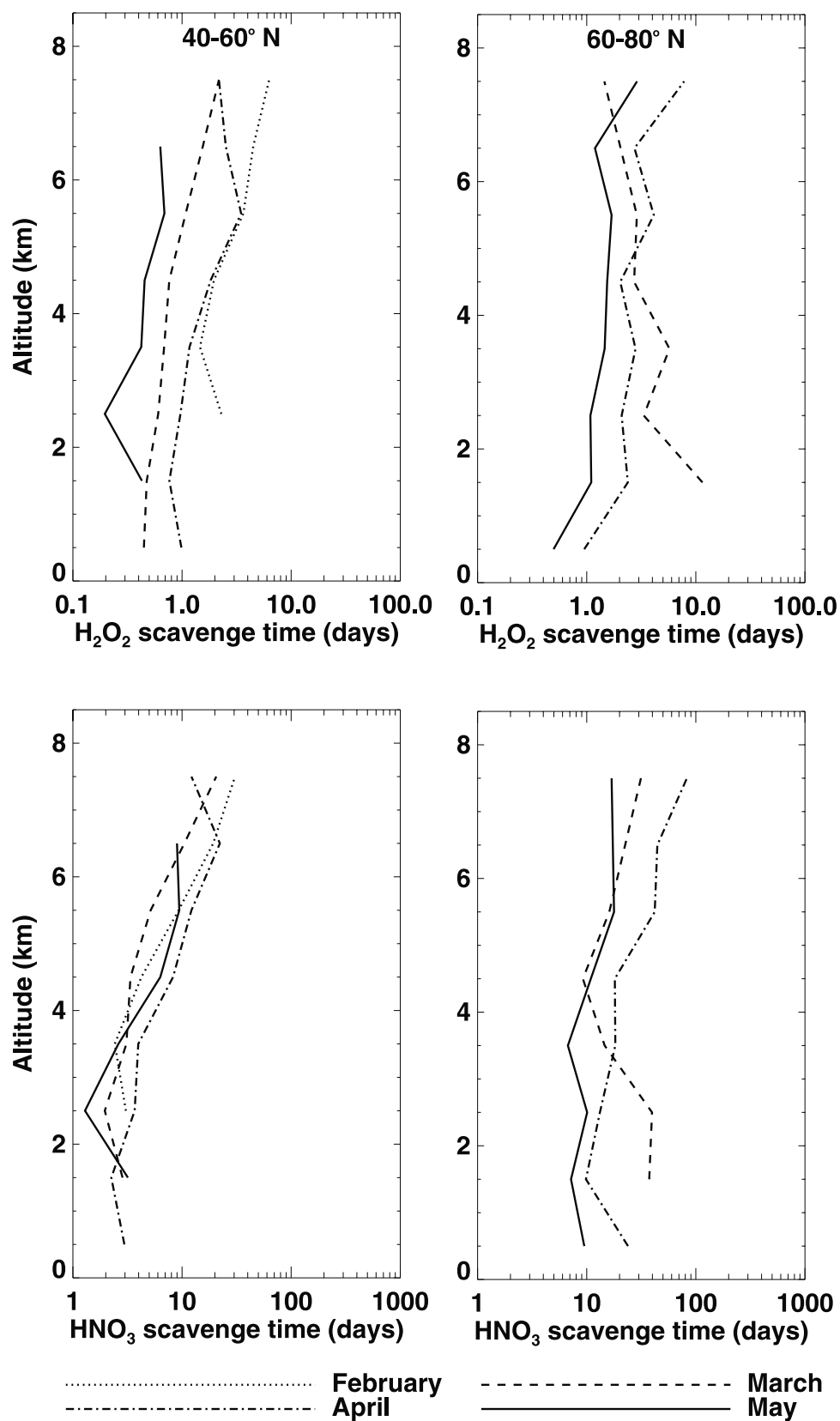
Figure 8. Same as Figure 1 but for estimated scavenging timescales of \text{H}_2\text{O}_2 and \text{HNO}_3 necessary to explain the observed concentrations.
