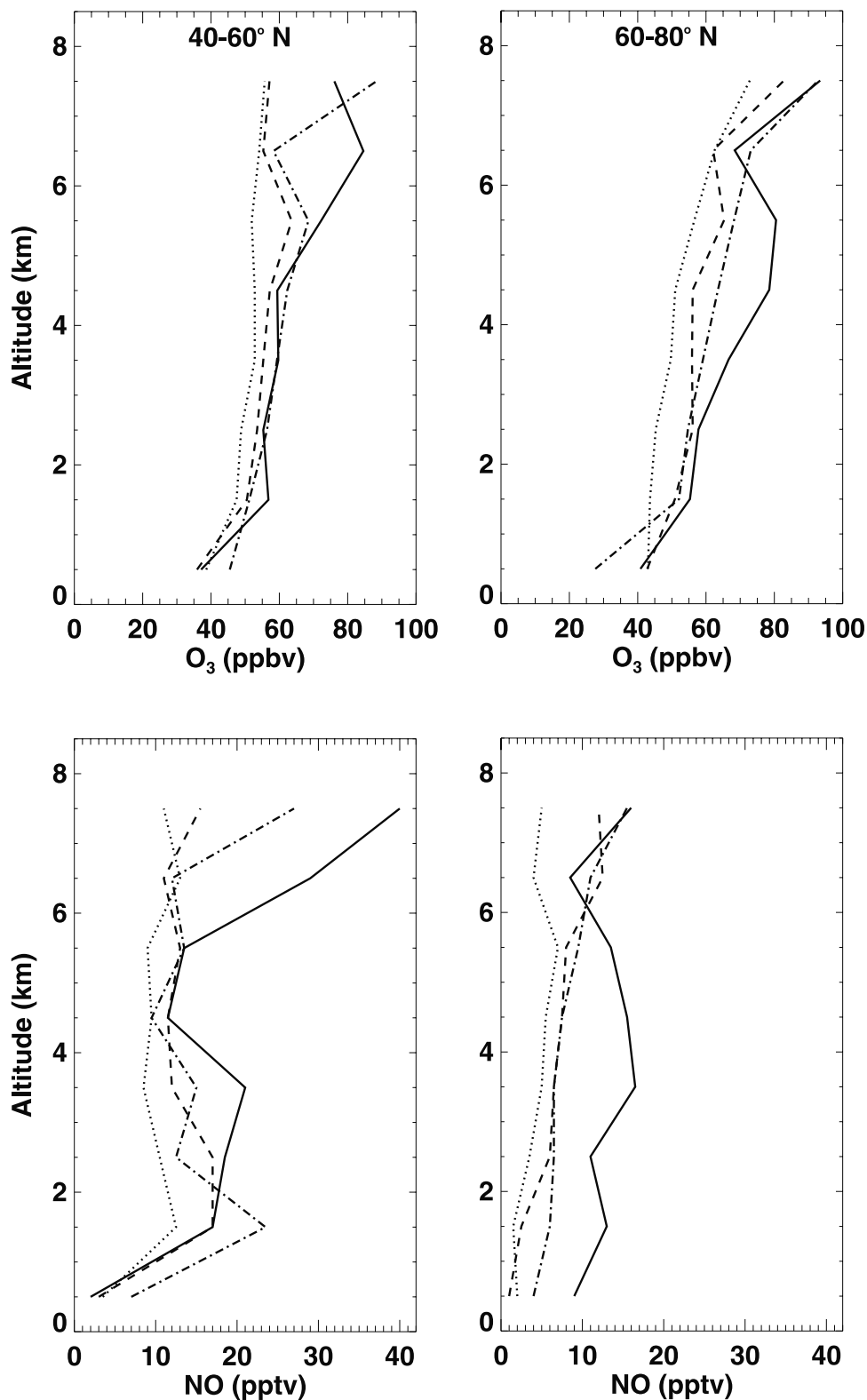
Figure 1. Monthly median profiles of observed \text{O}_3 , NO, \text{C}_2\text{H}_2 , and CO concentrations at mid ( 40^\circ – 60^\circ\text{N} ) and high latitudes ( 60^\circ – 80^\circ\text{N} ). Data are binned vertically in 1-km intervals. A median value plotted represents a minimum of 10 data points.
