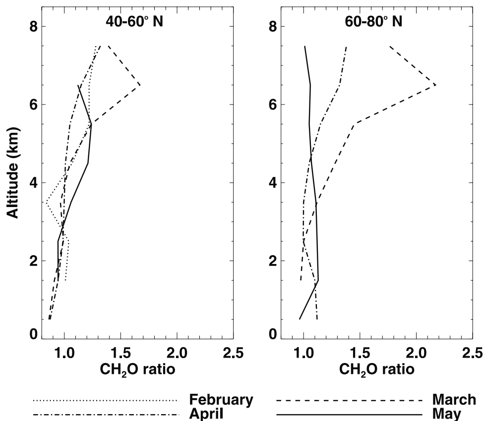
Figure 11. The monthly median ratios of simulated \text{CH}_2\text{O} concentrations with relative to without constraining \text{CH}_3\text{OOH} to observed values in the model. Each median value represents a minimum of 5 data points. The model is constrained by observed \text{H}_2\text{O}_2 concentrations.
