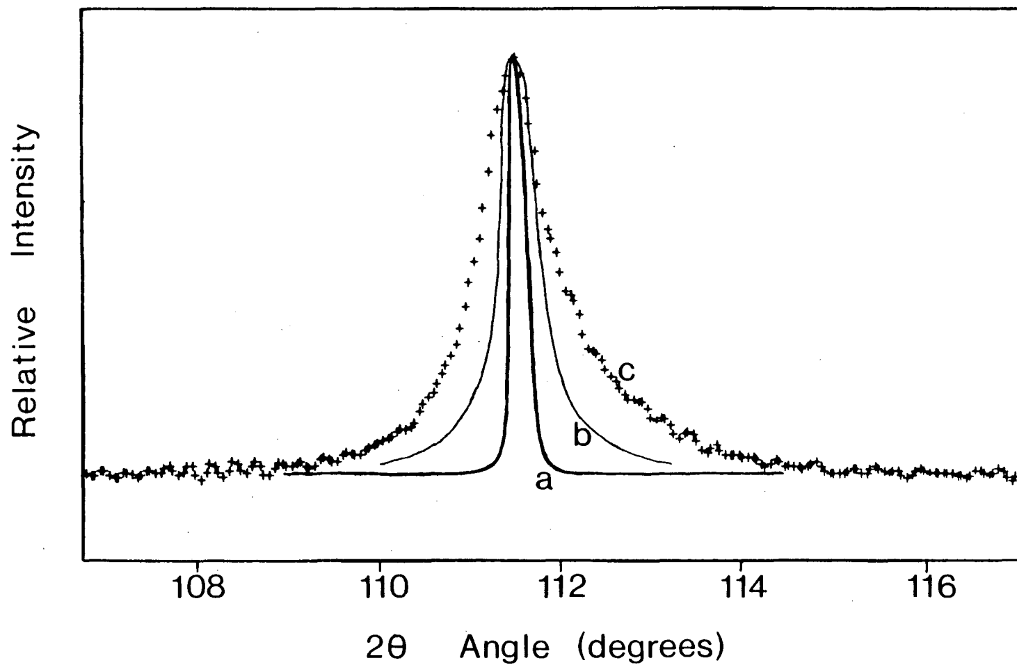
Fig. 1. Representative Rachinger and Stokes corrected (211)\alpha' XRD peaks from 9 Ni steel. a) dark line: 9 hr tempering at 590^\circ\text{C} , quench to 0^\circ\text{C} . b) light line: 240 hr tempering at 590^\circ\text{C} , quench to 0^\circ\text{C} . c) crosses: 240 hr tempering at 590^\circ\text{C} , quench to 0^\circ\text{C} , 75% cold rolling.
