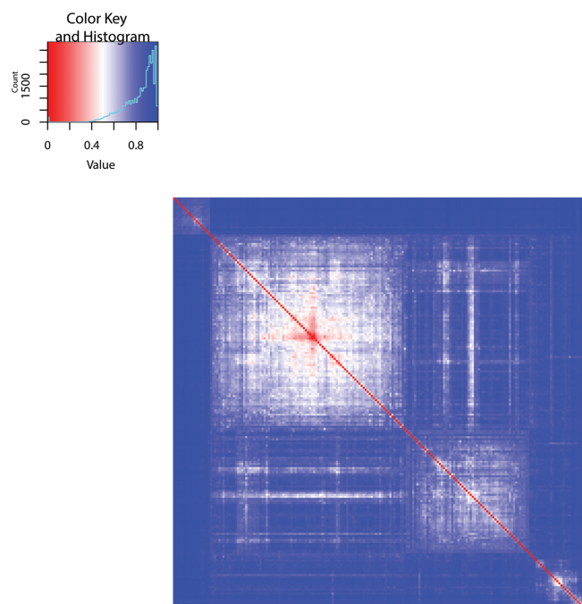
Figure 8. Heatmap of pairwise distances of the top 200 regions, identified by the horizontal alignment on ESC sample E003. Based on the distance matrix D , the top 200 regions are grouped into four clusters by average-linkage hierarchical clustering.
