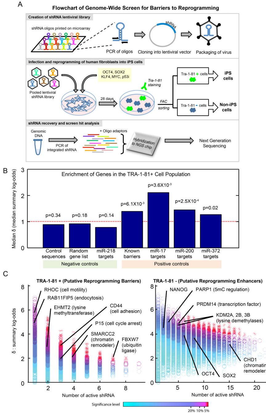
Figure 1. A Genome-Wide RNAi Screen Identifies Known and Novel Regulators of Human iPSC Generation
