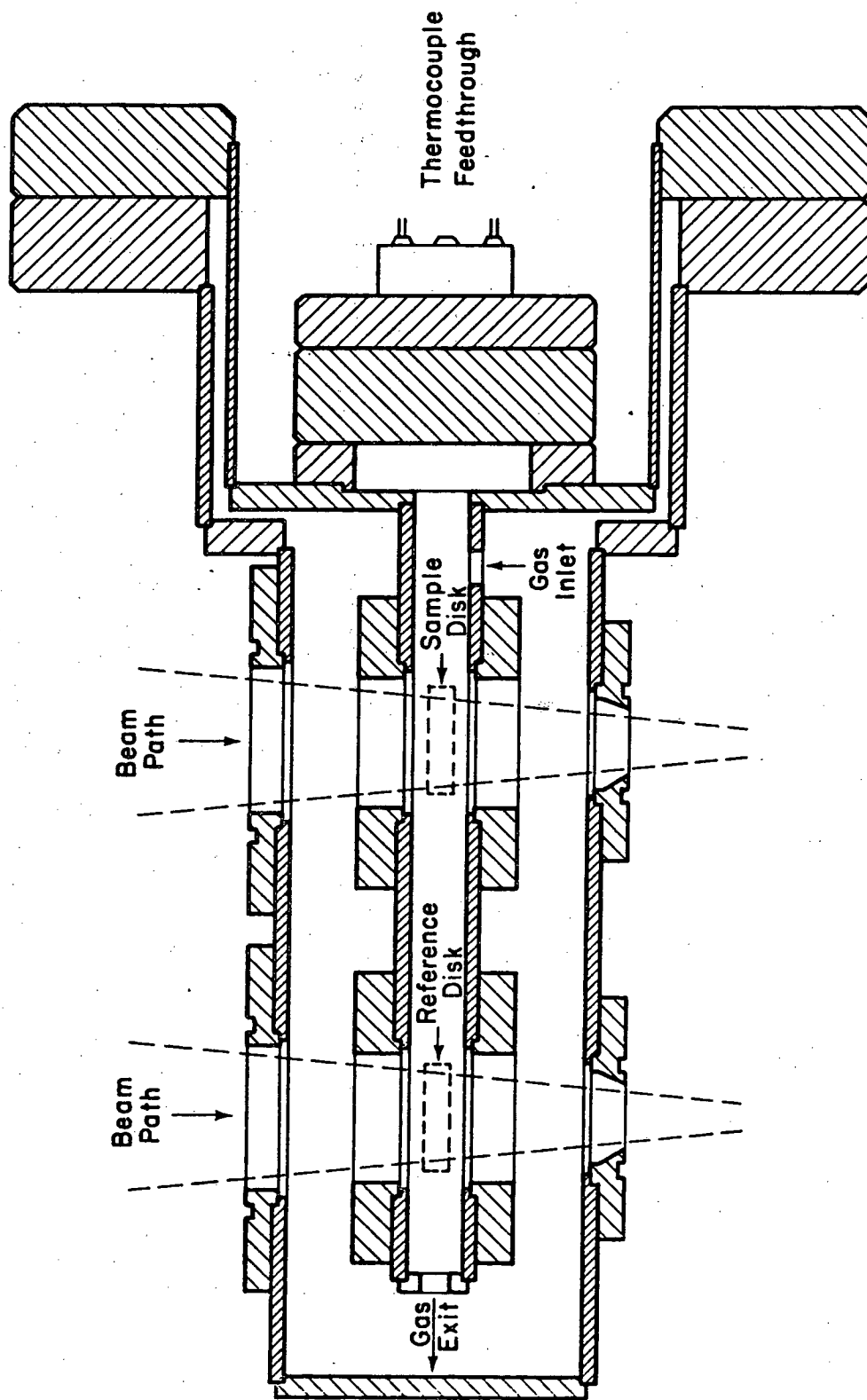
Figure 2. Reactor cross-sectional view
