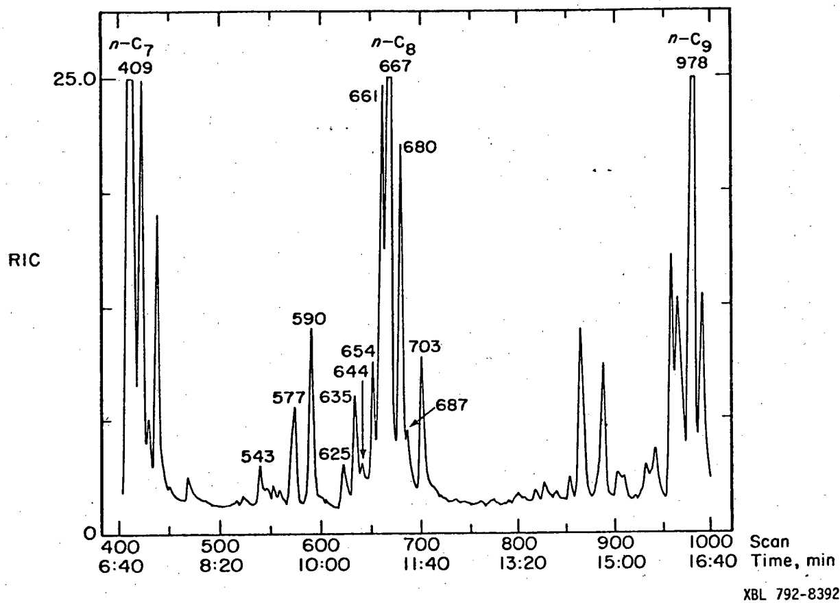
Figure 23. Chromatogram of the synthesis products
