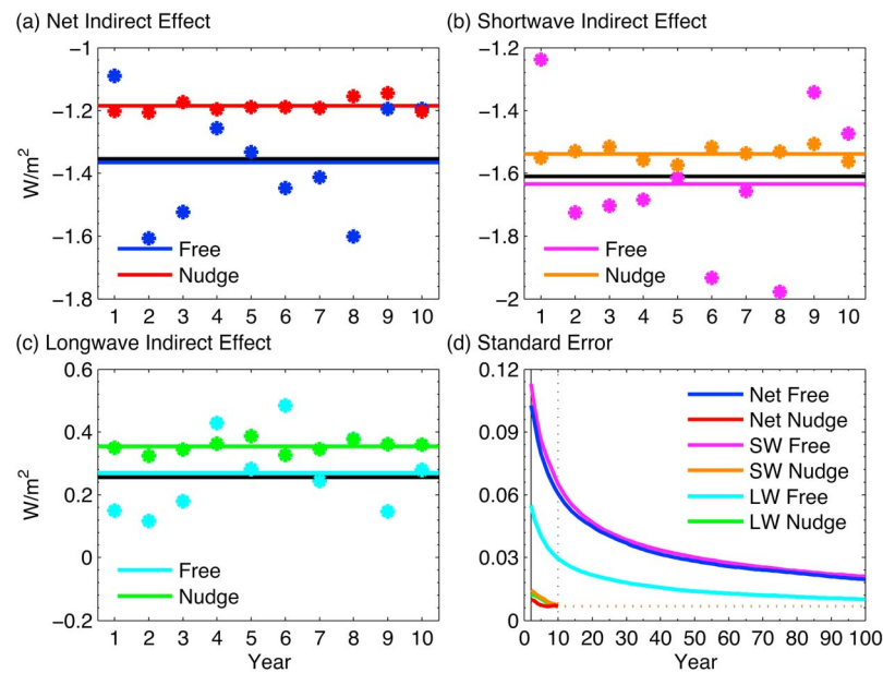
Figure 2. The global annual mean (a) net, (b) shortwave, and (c) longwave cloud forcing difference between present-day and pre-industrial (aerosol indirect effect) in CAM5 for each simulation year and (d) the standard error as a function of the number of sample years. The solid lines in Figures 2a–2c indicate 10-year mean values and the black solid line indicates the 100-year mean value from the free-running simulation.
