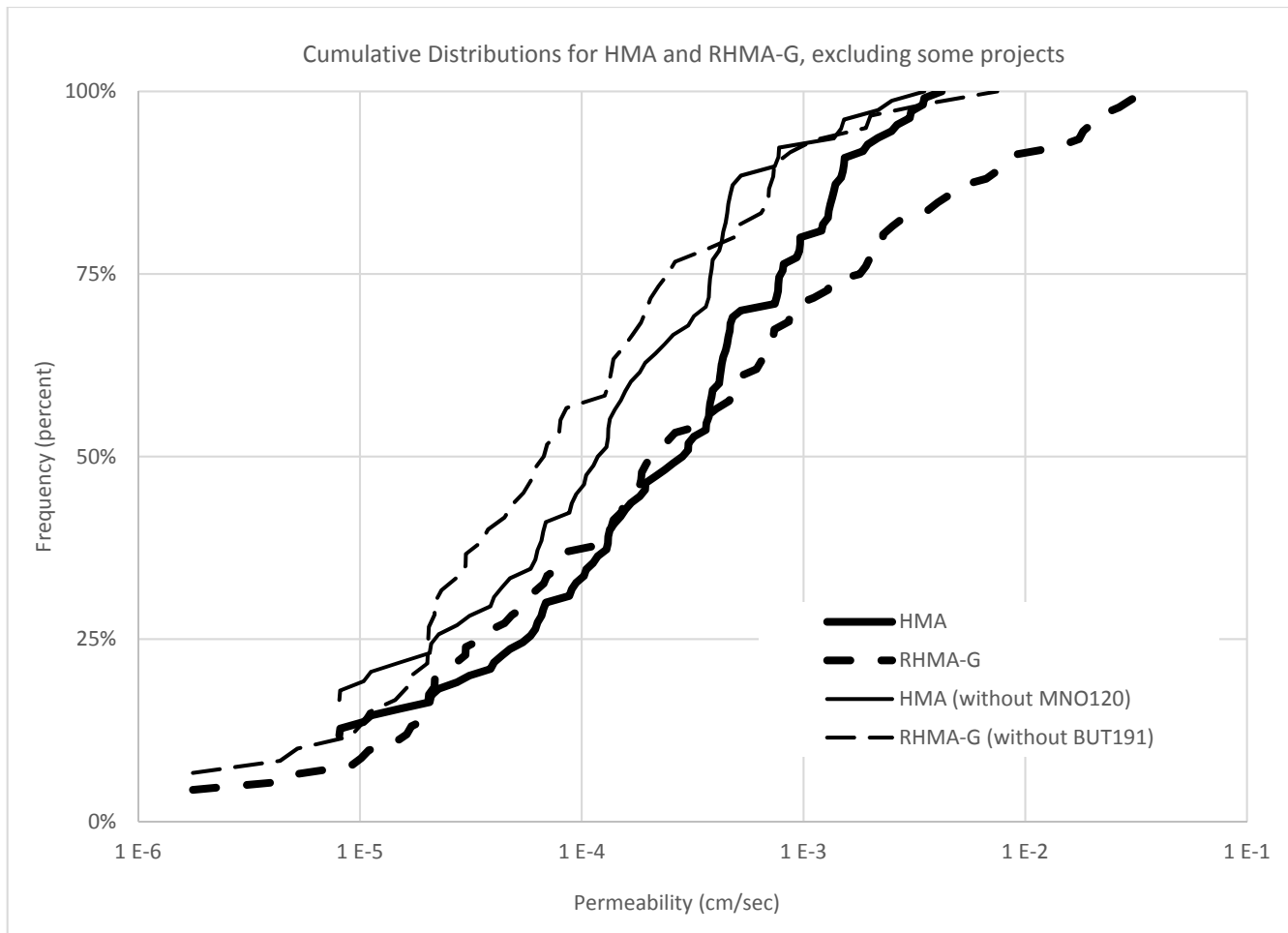
Figure 2.5: Cumulative distributions for the HMA data and RHMA-G data, excluding some projects.
