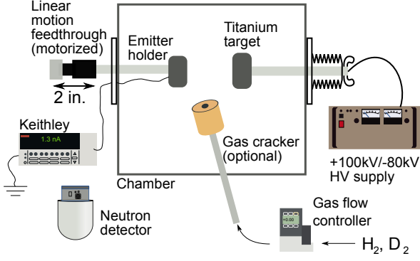
FIG. 3. (Color online) Schematic of the experimental setup for the high-voltage experiments.
