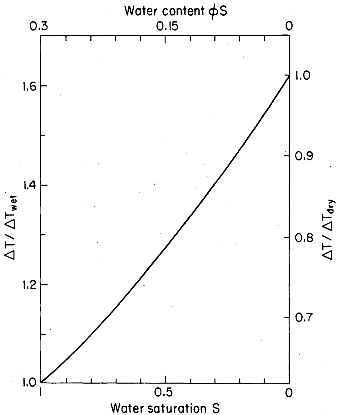
Figure A14. Increase in repository temperature in a dry rock medium based on geometric mean model. [XBL 8111-4883]
