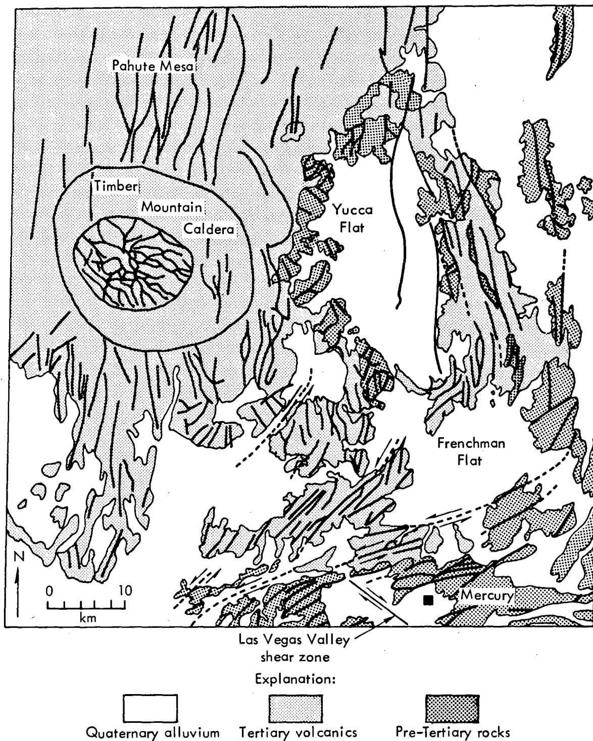
Figure 6. Map showing pattern of Basin and Range faults in Nevada Test Site and vicinity (after Ekren, 1968, from Borg et al., 1976). [XBL 832-8111]
