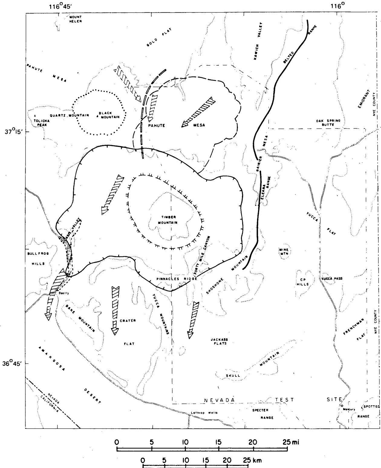
Figure 32. Map showing direction of groundwater movement from eastern Pahute Mesa toward discharge areas in Oasis Valley and Amargosa Desert, Nye County, Nevada (from Blankennagel and Wier, 1973).
