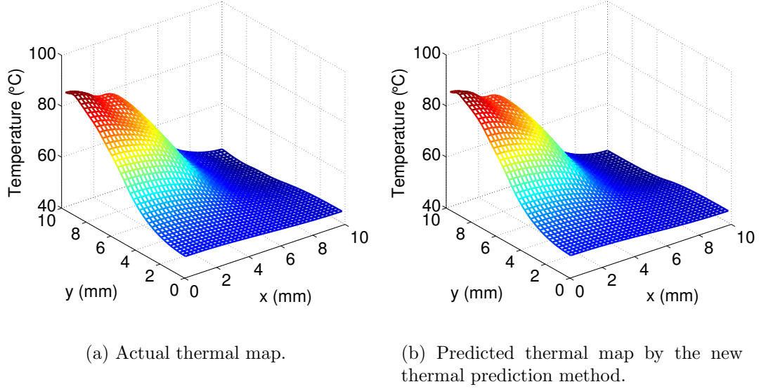
Figure 5.13: Accuracy of the predicted full-chip thermal map of bzip2 benchmark at 15s.
