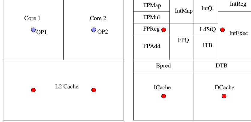
(a) The dual-core microprocessor architecture.
