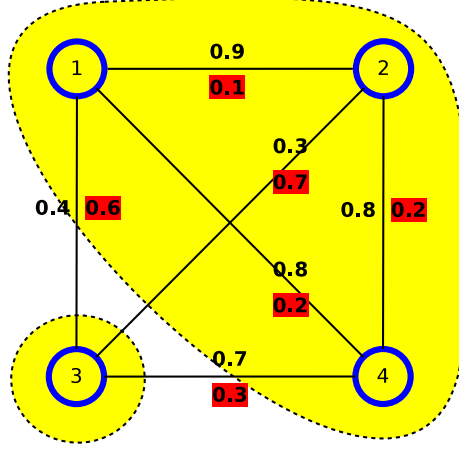
Figure 5.4: A correlation clustering example for a complete undirected weighted graph with four vertices. On each edge e_{ij} , w^-_{ij} is shown as red shaded while w^+ is in normal. The outputed clusters are surrounded by dashed lines filled with yellow color.
