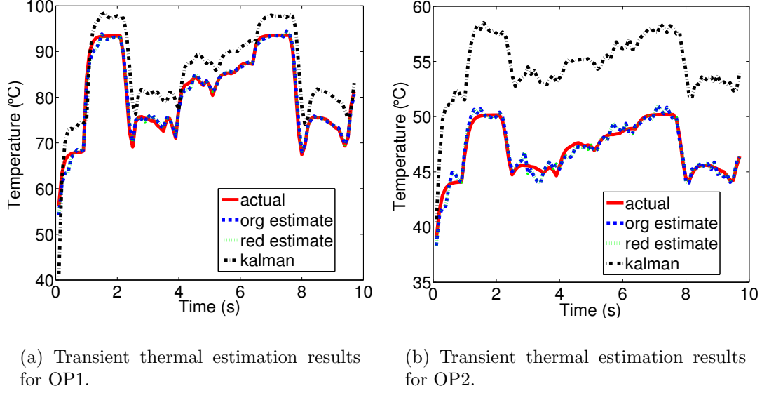
Figure 5.9: Transient thermal estimation results of bzip2 benchmark, where org represents the new method with original model before MOR, red represents the new method with reduced model after MOR and Kalman represents the Kalman filter based method [58].
