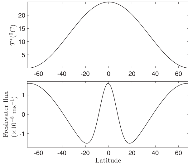
FIG. 2. (top) Relaxation temperature to which the model surface temperature is relaxed on a time scale of 15 days. (bottom) Surface freshwater flux. The salinity (virtual) flux imposed at the model's surface is the negative of the freshwater flux, multiplied by the reference salinity (35 psu).
