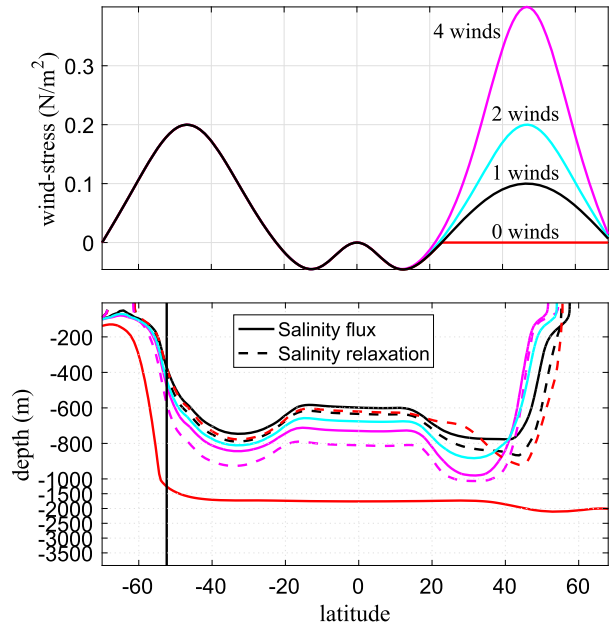
FIG. 3. (top) The wind stress profiles used in the computations as a function of latitude, labeled with the names used in subsequent figures. (bottom) Contours of the zonally averaged potential density surfaces \sigma_2 = 37 \text{ kg m}^{-3} in the latitude–depth plane for the different wind stress profiles, with colors matching the wind profiles of the top panel. Solid lines are for the experiments with fixed flux salinity boundary condition, and dashed lines are for the relaxation boundary condition.
