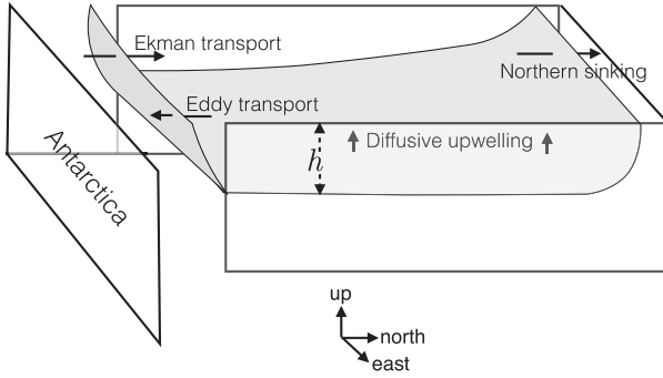
FIG. 1. Geometry of the conceptual model illustrating the budget for the residual circulation above the \sigma_2 = 37 \text{ kg m}^{-3} surface in the middepth MOC.
