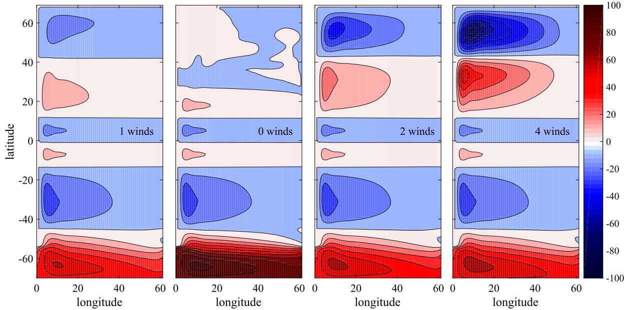
FIG. 7. Barotropic streamfunction (Sv) associated with the vertically integrated velocity for four computations forced by the different wind stress profiles given in the top panel of Fig. 3 and freshwater flux surface boundary condition. The contour interval is 10 Sv.
