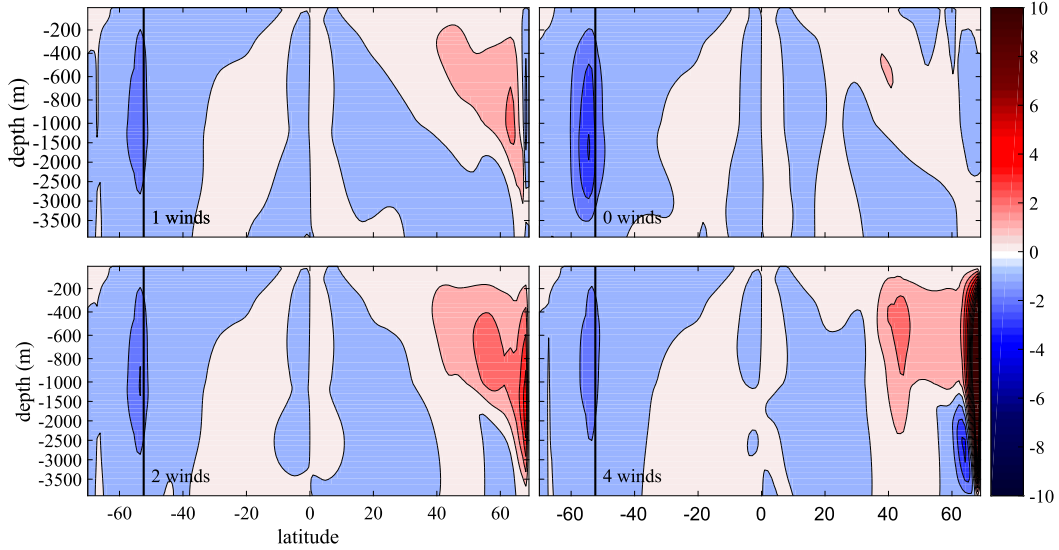
FIG. 5. Overturning streamfunction (Sv) associated with the time-averaged and zonal integral of the Gent–McWilliams bolus velocity (contour interval is 2 Sv), as a function of latitude and depth, for four computations forced by the different wind stress profiles given in the top panel of Fig. 3.
