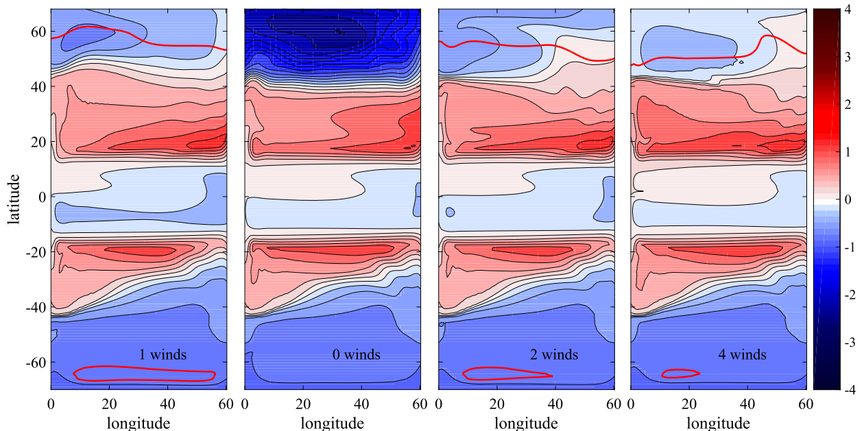
FIG. 8. SSS referenced to 35 psu for four computations forced by the different wind stress profiles given in the top panel of Fig. 3 and freshwater flux surface boundary condition. The contour interval is 0.2 psu. The thick red contour shows the position at the sea surface of the time-averaged \sigma_2 = 37 \text{ kg m}^{-3} (i.e., its time-averaged outcrop).
