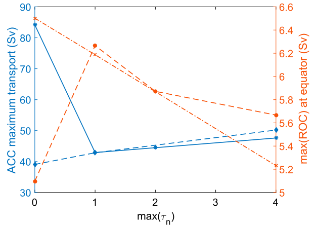
FIG. 6. Vertically and meridionally integrated zonal transport across the periodic portion of the domain (latitudes between 70° and 52.5°S) as a function of the maximum westerly wind stress amplitude in the Northern Hemisphere (blue lines; left axis): the blue solid line and asterisks are for the fixed flux boundary condition, and the blue dashed line and diamonds are for the relaxation boundary condition. Maximum residual transport across the equator as a function of the maximum westerly wind stress amplitude in the Northern Hemisphere (orange lines; right axis): the orange dashed line and circles are for the fixed flux boundary condition, and the orange dashed-dotted line and × marks are for the relaxation boundary condition.
