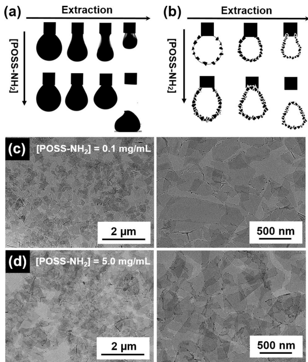
Figure 5. a) The images of the deformation and wrinkle behavior of the droplets at different \text{POSS-NH}_2 concentrations of 0.10 \text{ mg mL}^{-1} (top) and 5.0 \text{ mg mL}^{-1} (bottom). b) Schematics of the assembly of MXene surfactants at the interface during the extraction process at different \text{POSS-NH}_2 concentrations of 0.10 \text{ mg mL}^{-1} (top) and 5.0 \text{ mg mL}^{-1} (bottom). c, d) TEM images of the 2D MXene films with different \text{POSS-NH}_2 concentrations (the right image is the close-up view of the left image); [\text{Ti}_3\text{C}_2\text{T}_x] = 1.0 \text{ mg mL}^{-1} .
