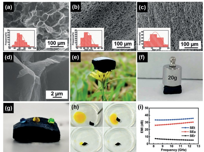
Figure 6. a–c) SEM images of MXene aerogels prepared from emulsion templates with different MXene concentrations of a) 2.0, b) 5.0, and c) 10 \text{ mg mL}^{-1} , [\text{POSS-NH}_2] = 1.0 \text{ mg mL}^{-1} ; d) close-up view of (c). e) A small piece of MXene aerogel on a flower; f) a small piece of aerogel (ca. 6.4 mg) supporting a 20g weight; g) water droplets on surface of MXene aerogel; h) oil absorption of MXene aerogel (the yellow oil phase is n -hexane dissolving azobenzene). i) EMI shielding performance of \text{Ti}_3\text{C}_2\text{T}_x @epoxy nanocomposite. Aerogels used in (e)–(i) are prepared in the case of [\text{Ti}_3\text{C}_2\text{T}_x] = 10 \text{ mg mL}^{-1} and [\text{POSS-NH}_2] = 1.0 \text{ mg mL}^{-1} .
