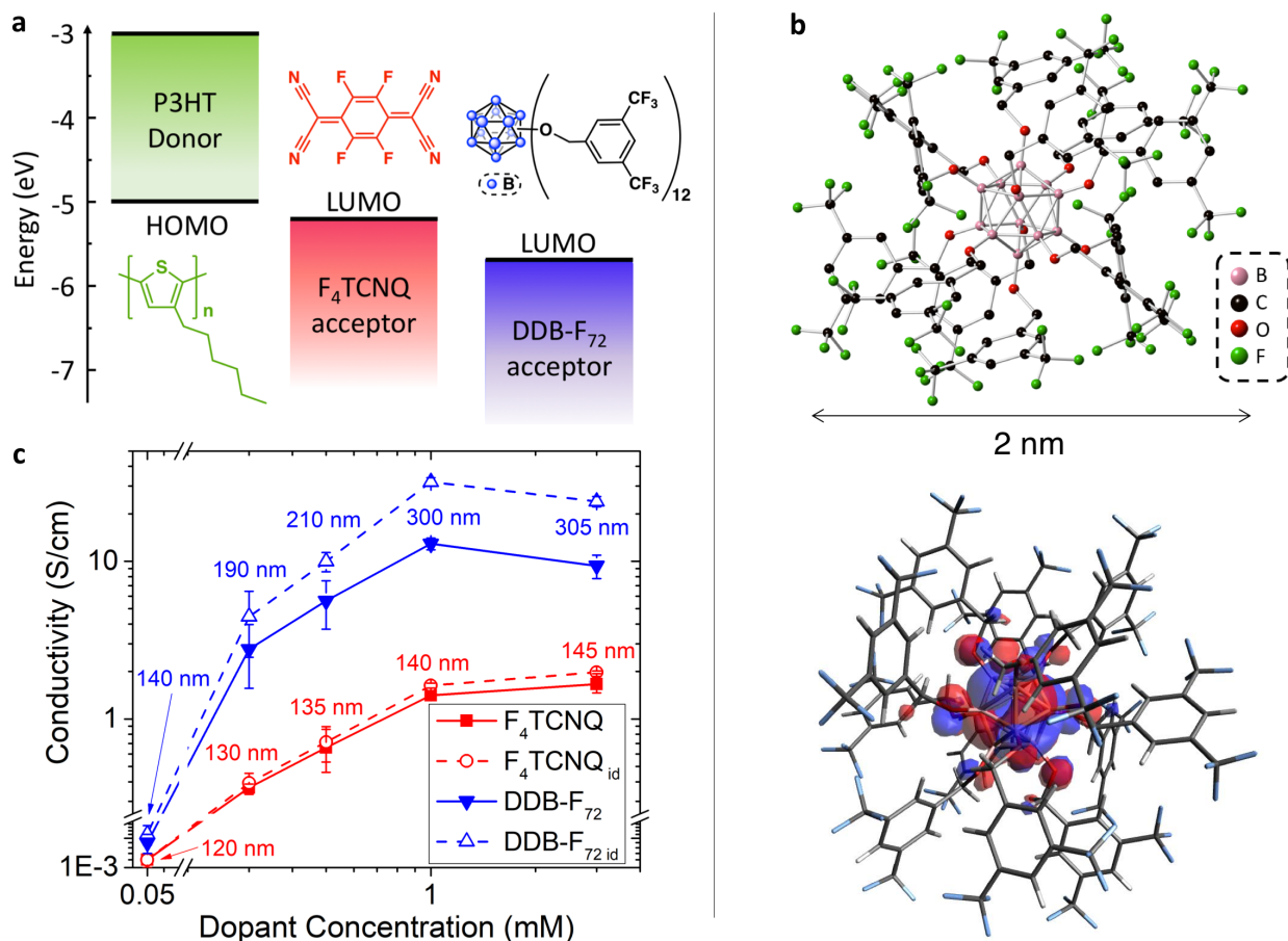
Figure 1. (a) Chemical structures and schematic energy diagram of P3HT, F 4 TCNQ, and DDB-F 72 showing \sim 0.5 V greater offset for DDB-F 72 than F 4 TCNQ. (b) (top) X-ray crystal structure of DDB-F 72 ; (bottom) DDB-F 72 anion SOMO calculated by TD-DFT showing the electron localized on the DDB core. (c) Conductivities (solid symbols, calculated using the measured thickness) and idealized conductivities (open symbols, calculated using the 120-nm original thickness) of P3HT films doped with F 4 TCNQ (red symbols) and DDB-F 72 (blue symbols) via solution sequential doping. The error bars are the standard deviation calculated from at least three samples. At the same dopant concentration DDB-F 72 produces conductivities that are an order of magnitude higher than those produced by F 4 TCNQ.
