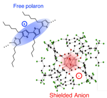
Figure 4. TOC graphic
