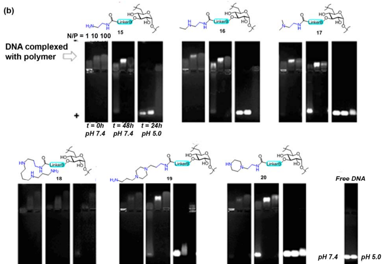
Figure 5.8. Complex formation between amine-dextrans and DNA at different N/P ratios, and release of DNA from the complexes at pH 7.4 and pH 5.0. a) Gel electrophoresis of complexes of DNA and slow-degrading amine-dextrans 9-14 at various time points. b) Gel electrophoresis of complexes of DNA and fast-degrading amine-dextrans 15-20 at various time points.
