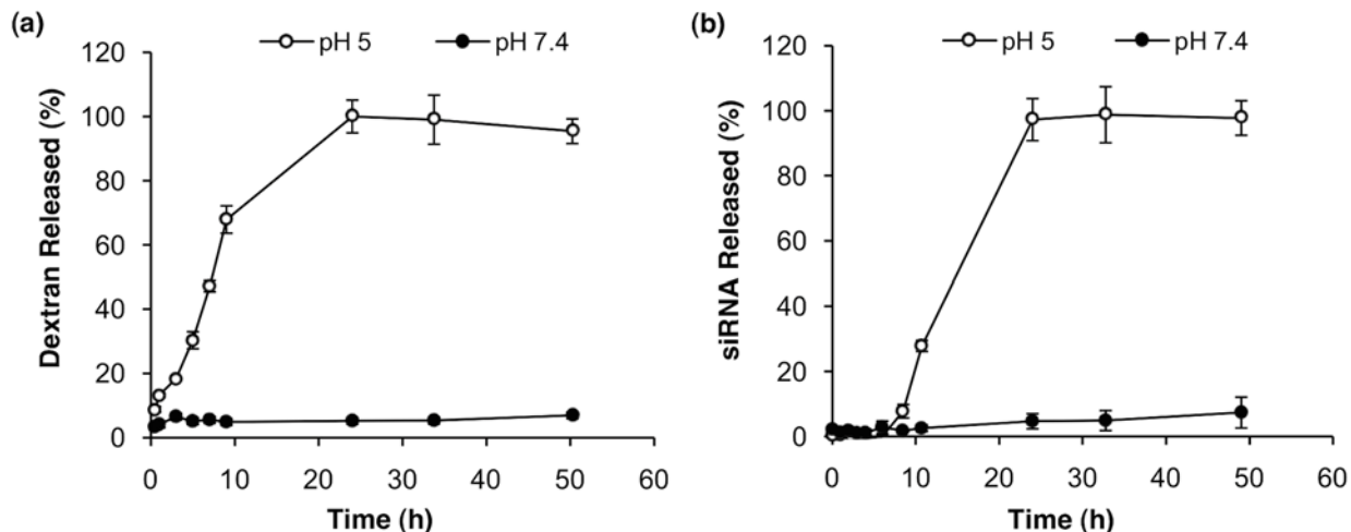
Figure 4.3. (a) Degradation of particles when incubated at pH 7.4 (black circles) and pH 5 (white circles), as determined by analysis of released soluble dextran. (b) Release of siRNA from spermine-Ac-DEX particles when incubated at pH 7.4 (black circles) or pH 5 (white circles). Data represent the mean \pm standard deviation of triplicate measurements.
