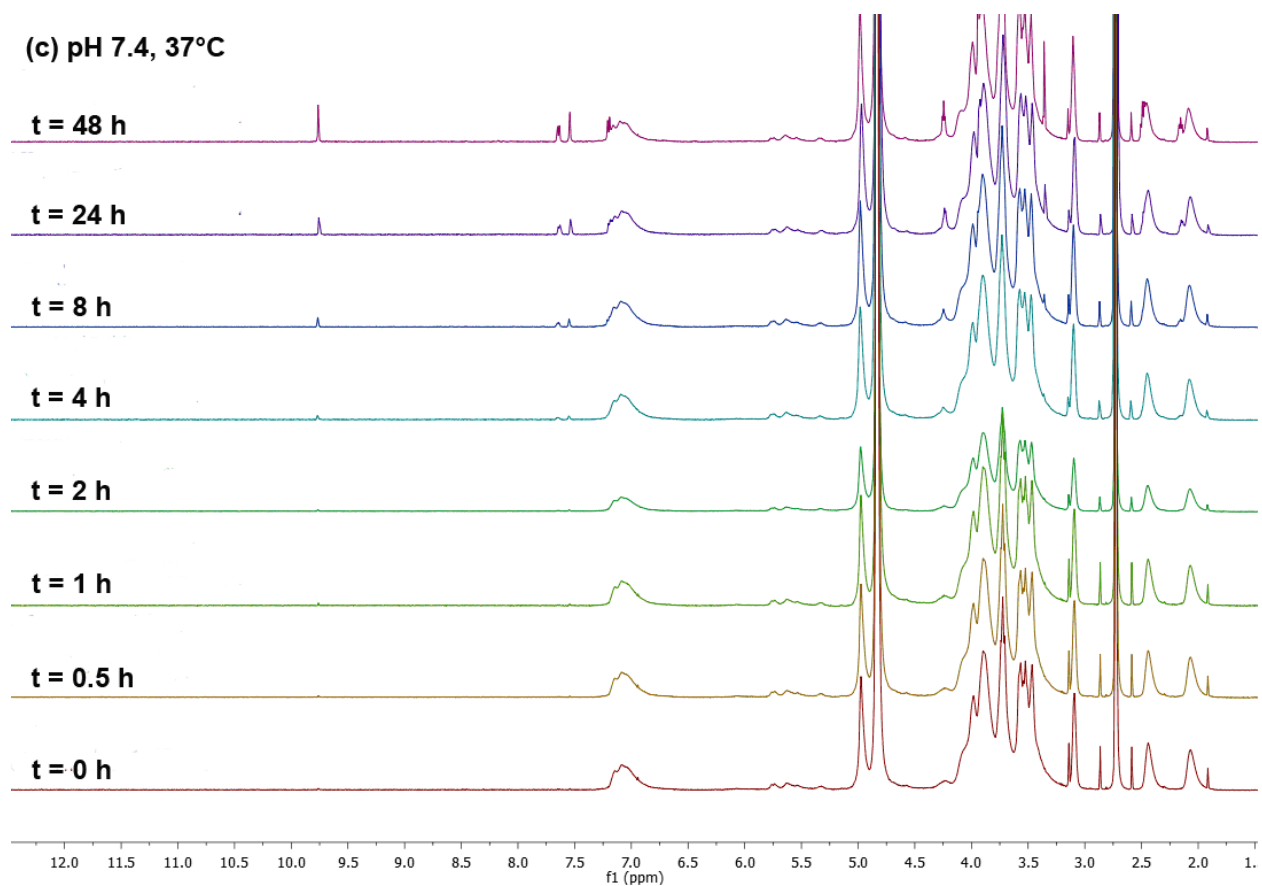
Figure 5.6. Degradation study of fast-degrading amine-dextran 15 * at 37°C. a) Scheme of the degradation reaction under acidic conditions. b) Array of ^1\text{H} NMR spectra of amine-dextran 15 at various incubation times (bottom to top: time = 0, 0.5, 1, 2, 4, 8, 24, 48 h) at pH 5.0. c) Array of ^1\text{H} NMR spectra of amine-dextran 15 at various incubation times (bottom to top: time = 0, 0.5, 1, 2, 4, 8, 24, 48 h) at pH 7.4.*For clarity, the degradation of the simplest fast-degrading amine-dextran 15 was shown. Other fast-degrading amine-dextrans degraded in roughly the same manner.
