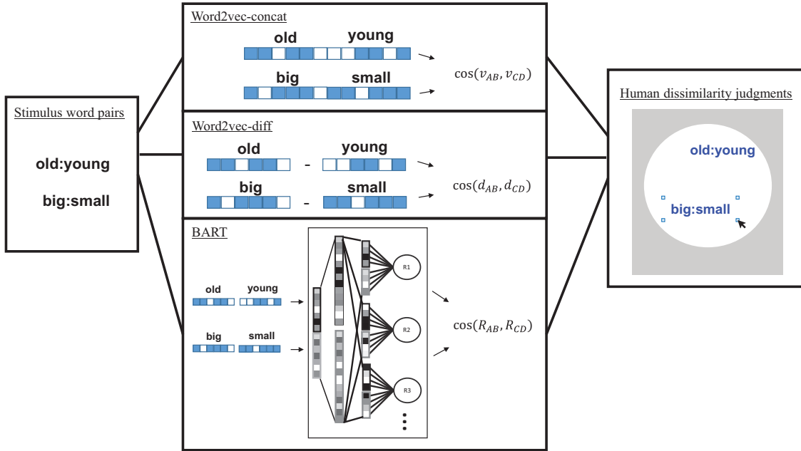
Figure 1 Schematic Illustration of Model-Generated Predictions of Human Dissimilarity Judgments Among Semantic Relations
