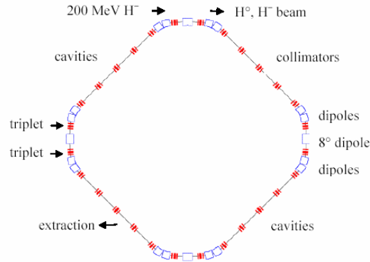
Fig. 2. Layout of 50 Hz, 3 GeV booster synchrotron.
