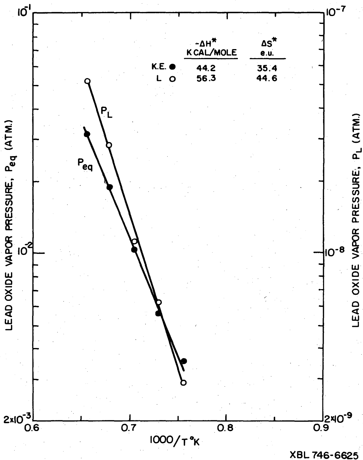
Figure 16. Lead oxide vapor pressure versus reciprocal temperature as determined by both the Langmuir equation and Knudsen effusion data.
