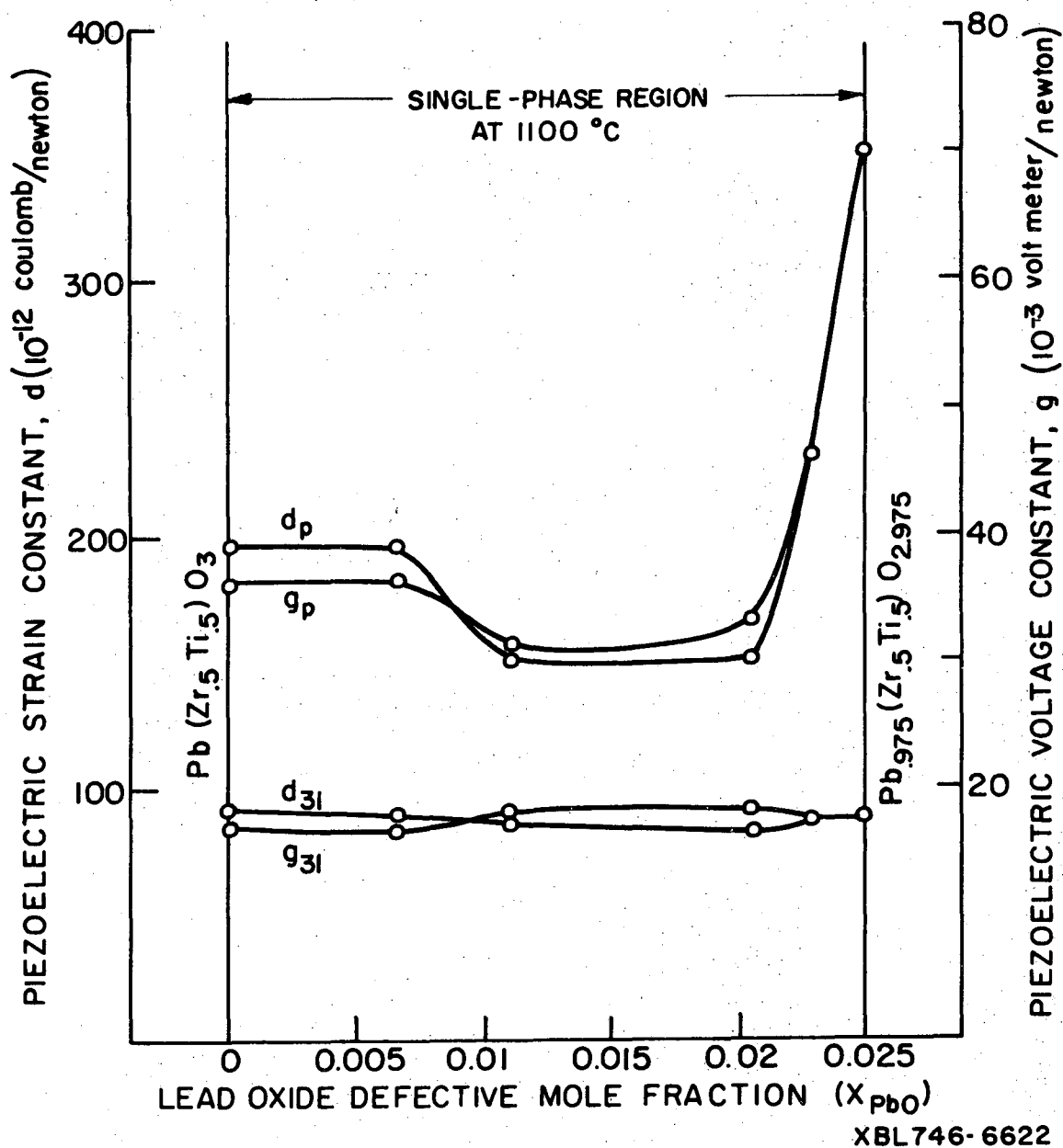
Figure 26. Piezoelectric parameter data versus lead oxide defective mole fraction at 1100°C.
