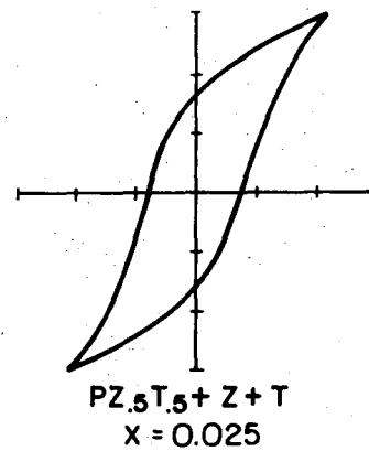
Figure 24. Ferroelectric hysteresis loops of \text{PZ}_{.5}\text{T}_{.5} where x equals the lead oxide defective mole fraction at 1100^\circ\text{C} .
