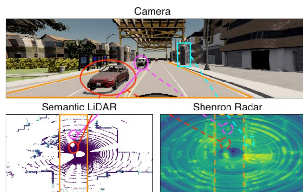
Figure 1: Illustrative image comparing views from Camera, Semantic LiDAR, and Shenron Radar in CARLA. Camera is in First Person View whereas LiDAR and Radar are in Birds Eye View perspective. The orange lines outline the road, red and magenta highlights vehicles, and blue indicates a static object.
