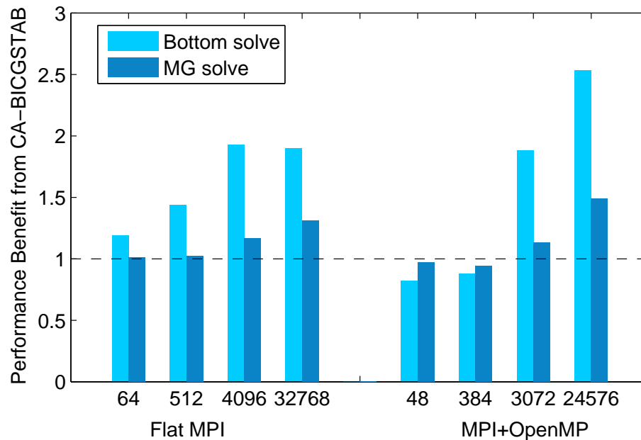
Figure 8.14: Speedup of mac_project using CA-BICGSTAB in the 3D version of LMC, as a function of the number of cores used and programming model.
