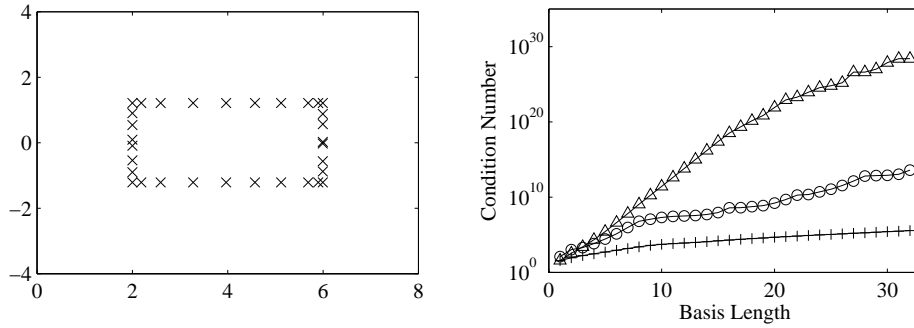
Figure 4.1: Basis properties for cdde . Left: computed Leja points ( \times ) of cdde , plotted in the complex plane. Right: basis condition number growth rate. The x-axis denotes basis length s and the y-axis denotes the basis condition number for monomial ( \triangle ), Newton ( \circ ), and Chebyshev ( + ) bases. Leja points on the left were used to generate the bases shown in the right plot.
