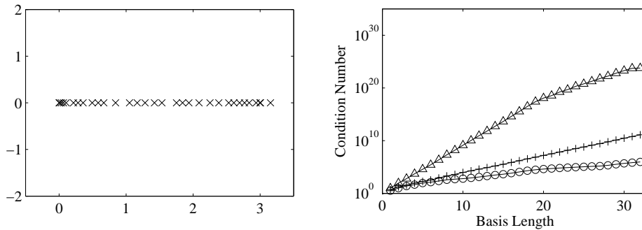
Figure 4.3: Basis properties for xenon1. Left: computed Leja points ( \times ) of xenon1, plotted in the complex plane. Right: basis condition number growth rate. The x-axis denotes basis length s and the y-axis denotes the basis condition number for monomial ( \Delta ), Newton ( \circ ), and Chebyshev ( + ) bases. Leja points on left were used to generate the bases shown in the right plot.
