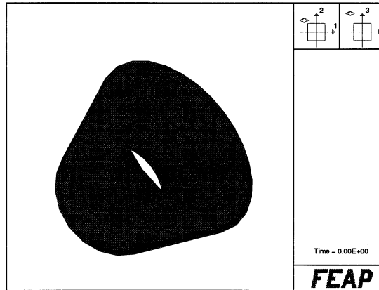
Figure 11. Torsional tube mesh from FEAP. Fixed grip boundary conditions were applied to the top and bottom of the tube for the axial driven problems; zero force boundary conditions were enforced for the axially free run.
