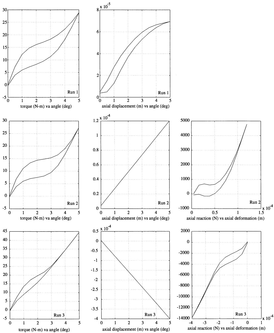
Figure 12. Combined torsion and axial loading of a cubic ↔ orthorhombic material tube. The left column of plots show the torque vs applied angle, the center column shows the applied axial displacement vs applied angle, and the right column plots give the axial response vs the axial deformation. The first row gives the results for free axial boundary conditions, the second gives the results for an applied extension, and the last row is for an applied compression. The units in all the plots are meters and newtons; the problem is described in the text and in Figure 11. The effect of axial loading on the pseudoelastic transformation, particularly compression in this example, is seen from the three simulations.
