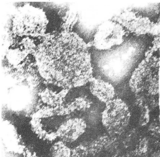
NEG.-STAINED MITOCHONDRIA (PARK and PACKER)
