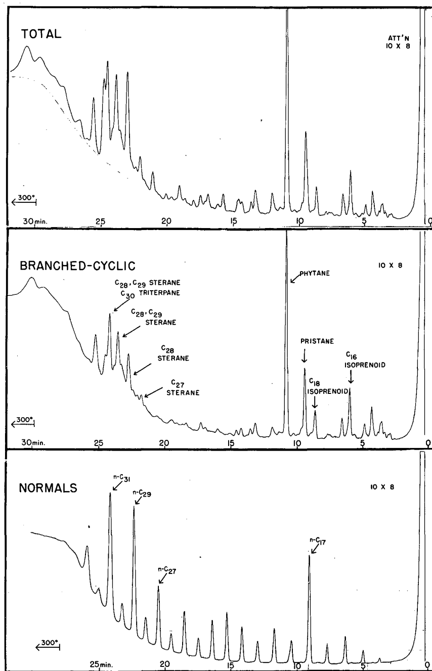
GREEN RIVER SHALE (COLORADO), \sim 60 \times 10^6 YRS. ALKANE FRACTIONS
