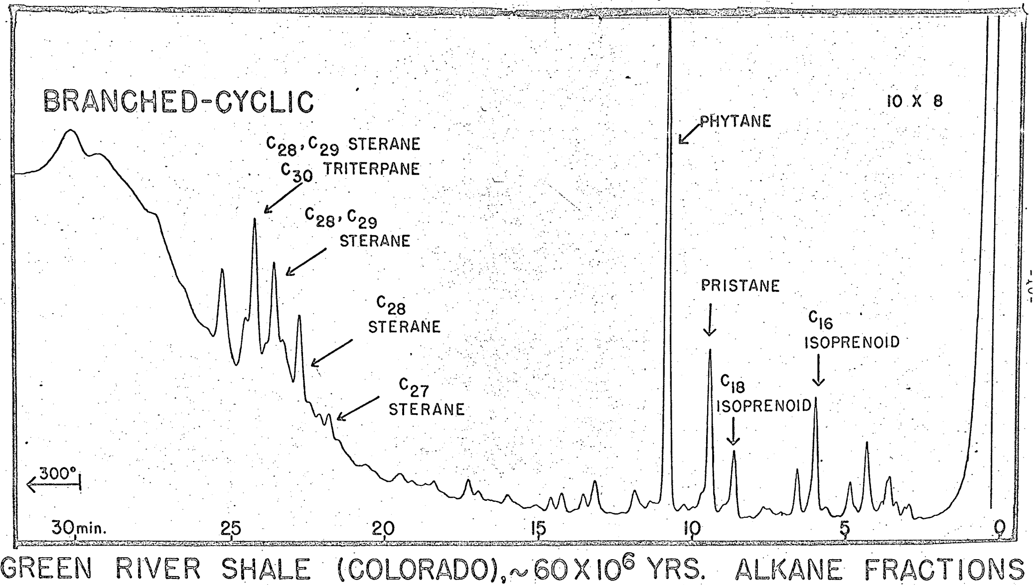
Figure 2a. Vapor phase chromatogram of branched-cyclic fraction, Green River Shale
