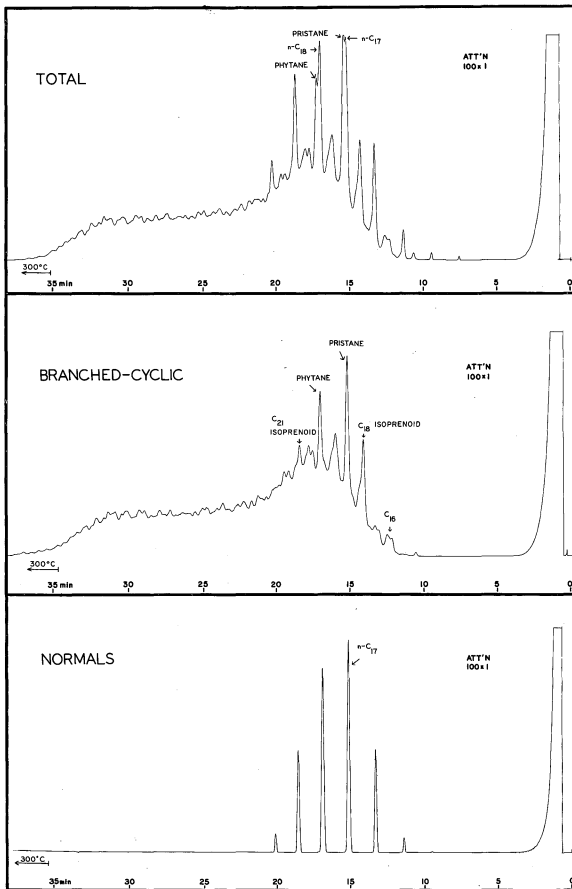
SUDAN SHALE ALKANE FRACTIONS
