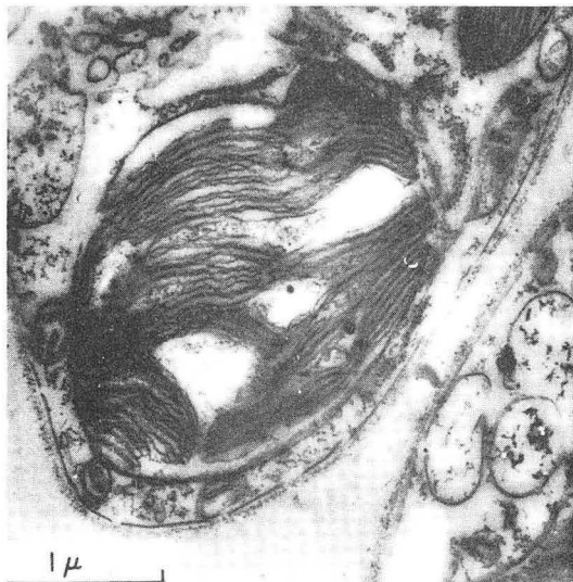
CHLOROPLAST WITH MITOCHONDRIA CHLAMYDOMONAS (SAGER)
