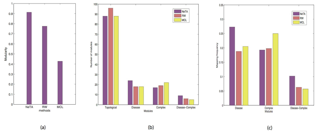
Figure 8. Systematic evaluation of NeTA based on a benchmark network. (a) The modularity of three clustering algorithms. (b) We mapped the detected topological modules to OMIM disease database and MIPS human complex database respectively, and counted the mapped number of disease modules, complex modules and disease-complex modules respectively, and compared them with the other two algorithms. (c) The mapped frequency of disease modules, complex modules and disease-complex modules respectively, in comparison with the other two algorithms.
