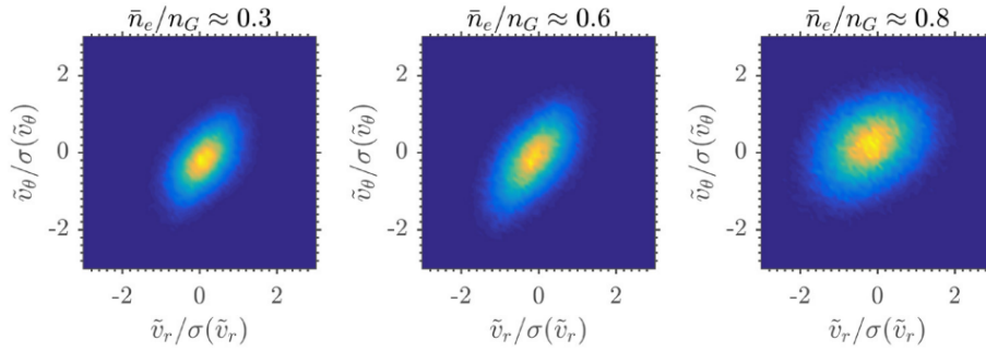
Figure 4. Joint probability distribution functions of \tilde{V}_r, \tilde{V}_\theta for three different densities near Greenwald density limit at r - r_{sep} = -1 cm. Note that as \bar{n}_e \rightarrow \bar{n}_G , the tilt of the pdf gradually lost and the symmetry of the turbulence restored. This indicates that shear flow production by Reynolds stress was weakened. This result is consistent with the drop in Reynolds power P_{Re} observed [5].
