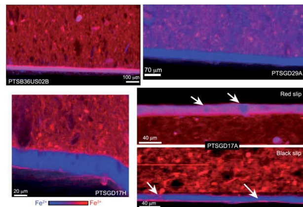
Fig. 3 Bicolor coded Fe valence state maps for the pre-sigillata recorded at SSRL (100% Fe 2+ in blue and 100% Fe 3+ in red). Arrows point the major Fe 2+ inclusions in Fe 3+ and inversely.
