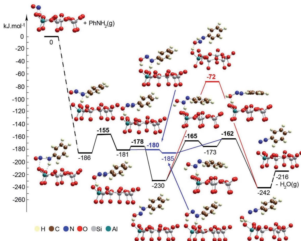
Fig. 9 Energy diagram and optimized models of the reaction steps for the \text{PhNH}_2 transformation in the pores of \text{Zeo}/\text{NO}^+ . The models are visualized with the VESTA program. 33
