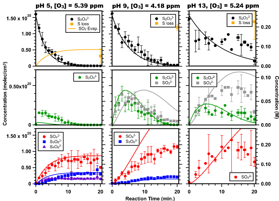
Figure 4. Representative detailed kinetics for the ozone oxidation of thiosulfate ( \text{S}_2\text{O}_3^{2-} ): thiosulfate decay (top panels), reaction intermediates (middle panels, y-scale zoomed for clarity) and reaction products (bottom panels) for pH 5 (left), pH 9 (middle) and pH 13 (right). Concentration is shown in molecular units on the left y-axes and in molar units on the right y-axis. Experiment results are shown as points representing the average of 5 individual runs with error bars representing the standard deviation of each set. The net loss calculated via sulfur closure is shown as ‘S loss’ (orange circle) in the top panels; see S9 in Supporting Information for more details. Simulation results are shown as lines. The calculated amount of \text{SO}_2 lost to the gas phase is shown as an orange line in the top panel for pH 5. Green points and lines represent both \text{S}_2\text{O}_4^{2-} and \text{HS}_2\text{O}_4^- as these cannot be distinguished in experiments. Species not shown for a given pH were not detected at a significant concentration by experiments and were not predicted to form at a significant concentration by simulations.
