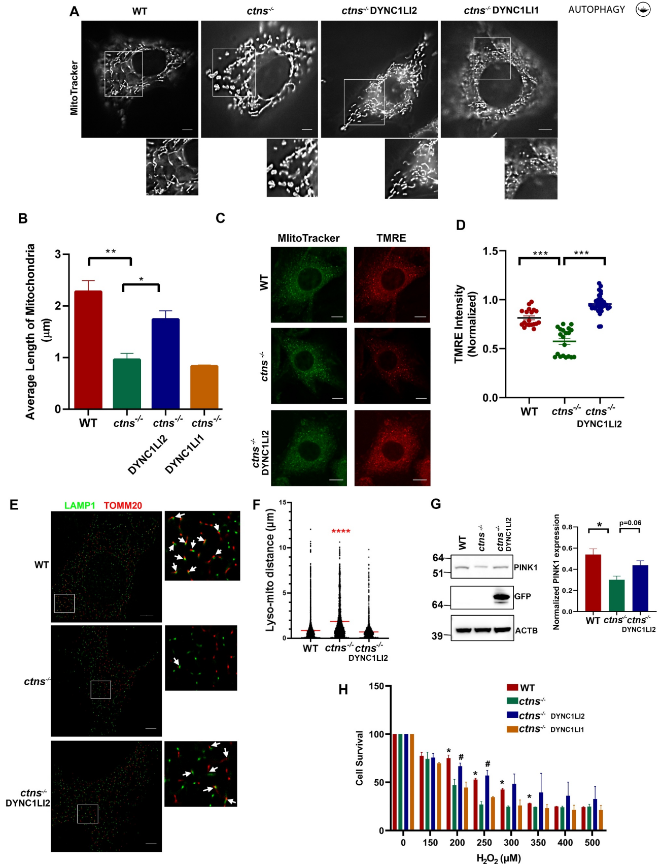
Figure 5. Reconstitution of DYNC1L12 but not DYNC1L11 expression decreases mitochondrial fragmentation and increases cell survival of ctns -/- cells. (A) Analysis of mitochondrial length in wild-type (WT), ctns -/- , DYNC1L12- and DYNC1L11-expressing ctns -/- cells by pseudo-TIRFM (oblique illumination) using MitoTracker. Scale bar: 6 \mu m. (B) Quantification of mitochondrial length. Mean \pm SEM, *, p < 0.05 ; **, p < 0.01 n = 3, 8-10 cells per experiment. (C and D) Analysis of mitochondrial membrane potential ( \Delta\psi_m ) by fluorescence microscopy. \Delta\psi_m was analyzed as the ratio between the fluorescence intensity of the probe TMRE (increased fluorescence in polarized mitochondria) normalized by MitoTracker (mitochondria mass indicator). (C) Representative images. (D) Quantitative analysis from 19 to 34 WT, ctns -/- , and GFP-DYNC1L12-expressing ctns -/- cells from 3 independent experiments. (E and F) Super resolution microscopy analysis of lysosomal-mitochondrial adjacency. (E) Representative images of cells labeled with anti-LAMP1 (green) and anti-TOMM20 (pseudo-colored red). Magnified images show areas with high lysosomal-mitochondria adjacency in WT and DYNC1L12-reconstituted ctns -/- cells (arrows) but low adjacency in ctns -/- cells. (F) Quantification of lysosomal mitochondria proximity. Pairs were plotted according to the distance to their most proximal counterpart. A total of 7202, 5778 and 4408 molecular pairs from 4 wild-type, ctns -/- , and DYNC1L12-reconstituted ctns -/- cells were analyzed by STORM. ****, p < 0.0001 . (G) Left panel, Immunoblotting analysis of the expression of PINK1. See Figure S7 for total protein loading controls. Right panel, Quantitative analysis of PINK1 expression from 3 independent experiments. Mean \pm SEM, Student's t-test. (H) GFP-DYNC1L11 and GFP-DYNC1L12-reconstituted MEFs were treated with H 2 O 2 and cell viability was analyzed by the MTT assay. Mean \pm SEM from 3 independent experiments performed in triplicates. *, p < 0.05 , WT vs ctns -/- ; #, p < 0.05 , ctns -/- vs DYNC1L12.
