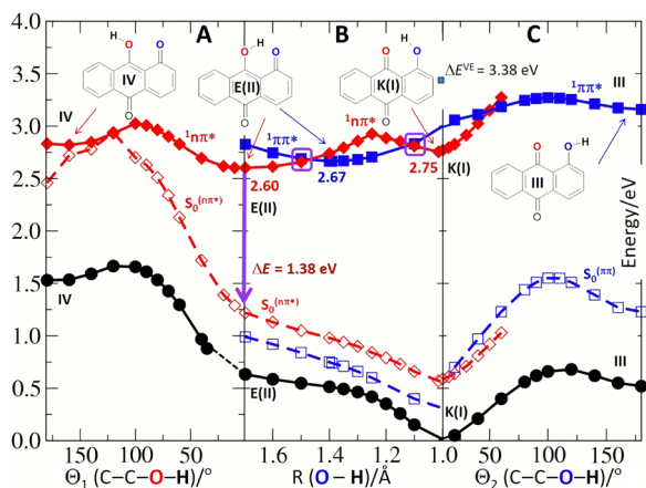
Fig. 5. Potential energy profiles of 1-HAQ. Profiles shown are of the S_0 state (black circles), the S_1(\pi\pi^*) state (blue squares), and the S_1(n\pi^*) state (red diamonds) of the 1-HAQ molecule as a function of the torsional reaction path (A and C) and the hydrogen transfer reaction path (B). Full lines (full symbols): Energy profiles of reaction paths determined in the same electronic state. Dashed lines (empty symbols) represent ground-state energy calculated for the geometry optimized in the given excited state n\pi^* (red) or \pi\pi^* (blue). Purple rectangles highlight the n\pi^* and \pi\pi^* intersections.
