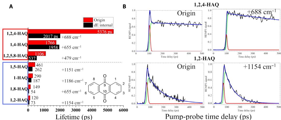
Fig. 3. Results of picosecond pump-probe spectroscopy. (A) Pump-probe lifetime as measured at the origin transition (red bars) and at excess energy (black bars) arranged in order of decreasing measured lifetimes. The excess energy transition used is noted next to the black bars. (B) Pump-probe traces of the molecules with the longest and shortest measured excited state lifetime, 1,2,4-HAQ and 1,2-HAQ, respectively, plotted over 500 ps. The pump-probe data are fit to a curve (blue trace), which is the sum of a single exponential decay (green trace) convolved with a Gaussian component (red trace) representative of our instrument response function.
