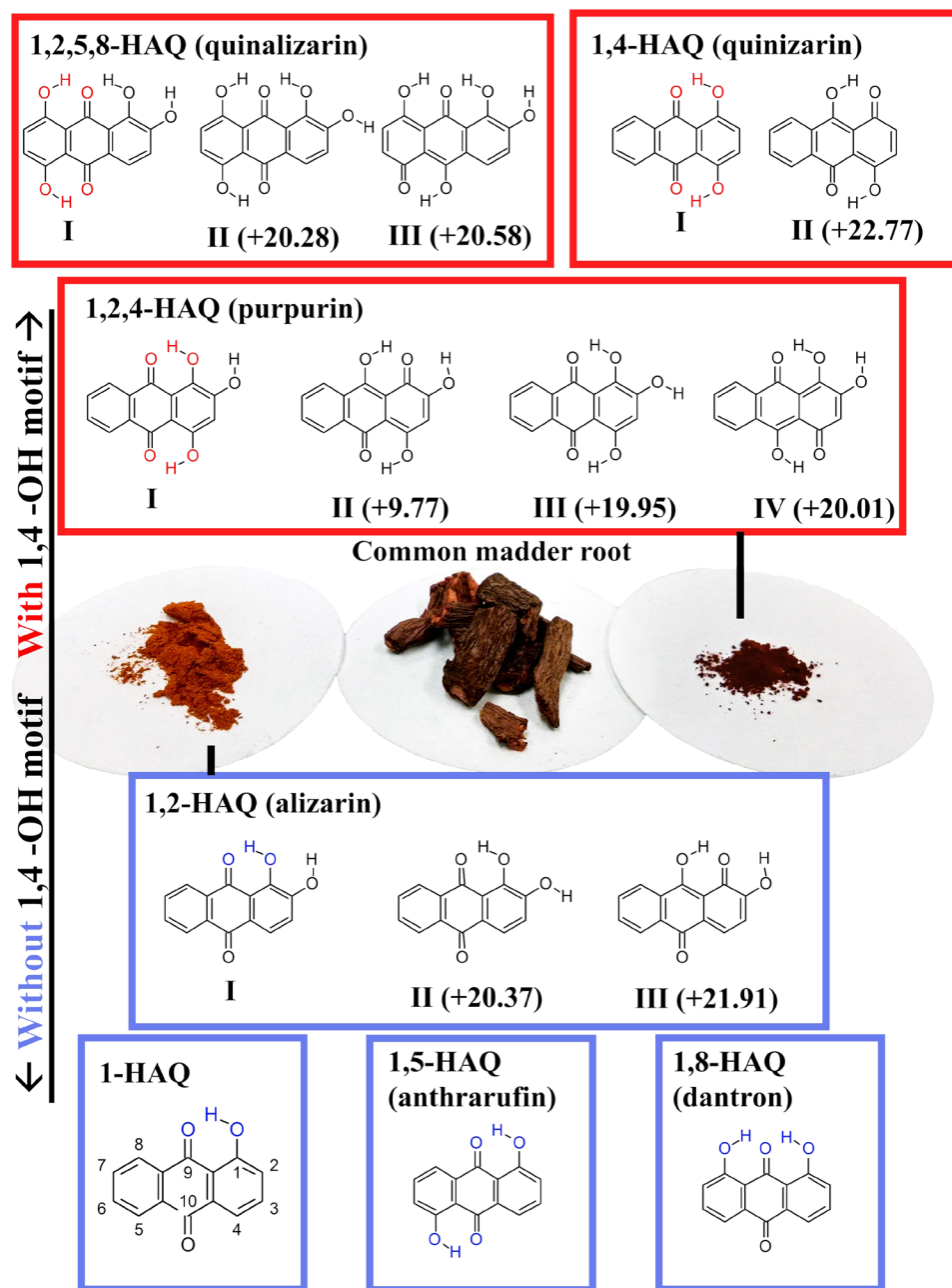
Fig. 1. The molecules of this study. Molecules having a 1,4-OH motif are above the images, and those without 1,4-OH motif are below them. Isomers within the LE ZPE corrected structure (labeled I) (~25 kJ/mol) are also shown with their relative energy values (kJ/mol) with respect to the LE form. Central to this figure is the common madder root and its primary chromophores alizarin and purpurin. Photo credit: Jacob Berenbeim, UCSB
