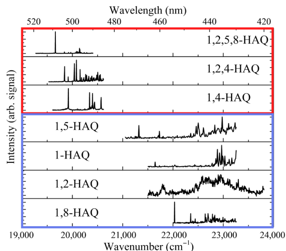
Fig. 2. Picosecond 2C-R2PI spectra of each HAQ in this study (OPG + 213 nm). Intensities have been normalized.
