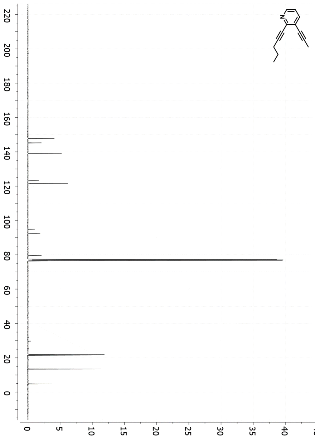
Figure 3.13. ^{13}\text{C}\{^1\text{H}\} NMR spectrum of 26 ( \text{CDCl}_3 , 100 MHz).
