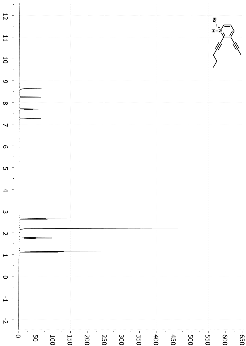
Figure 3.14. ^1\text{H} NMR spectrum of 32-Br ( \text{CDCl}_3 , 400 MHz).
