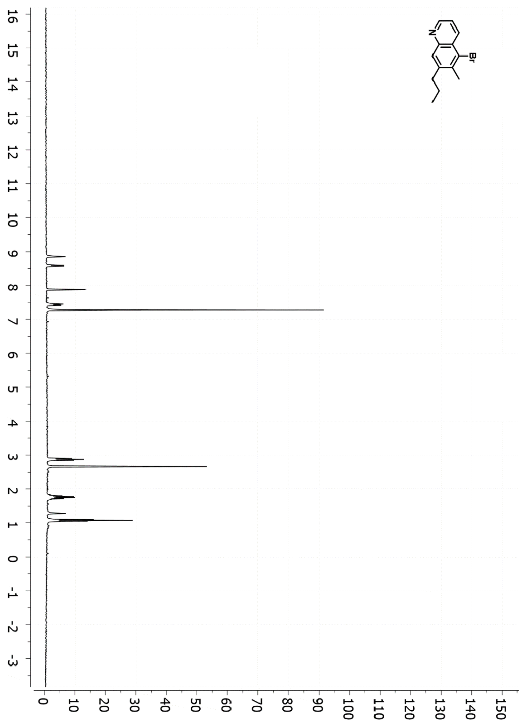
Figure 3.28. ^1\text{H} NMR spectrum of 29-Br ( \text{CDCl}_3 , 300 MHz).
