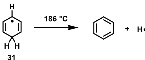
Scheme 3.10. Generation of a hydrogen radical from 31 . 17
