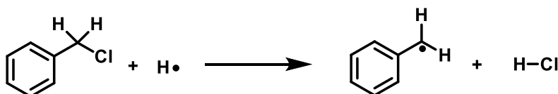
Scheme 3.11. HCl is formed via reaction of a hydrogen radical with benzyl chloride. 18
