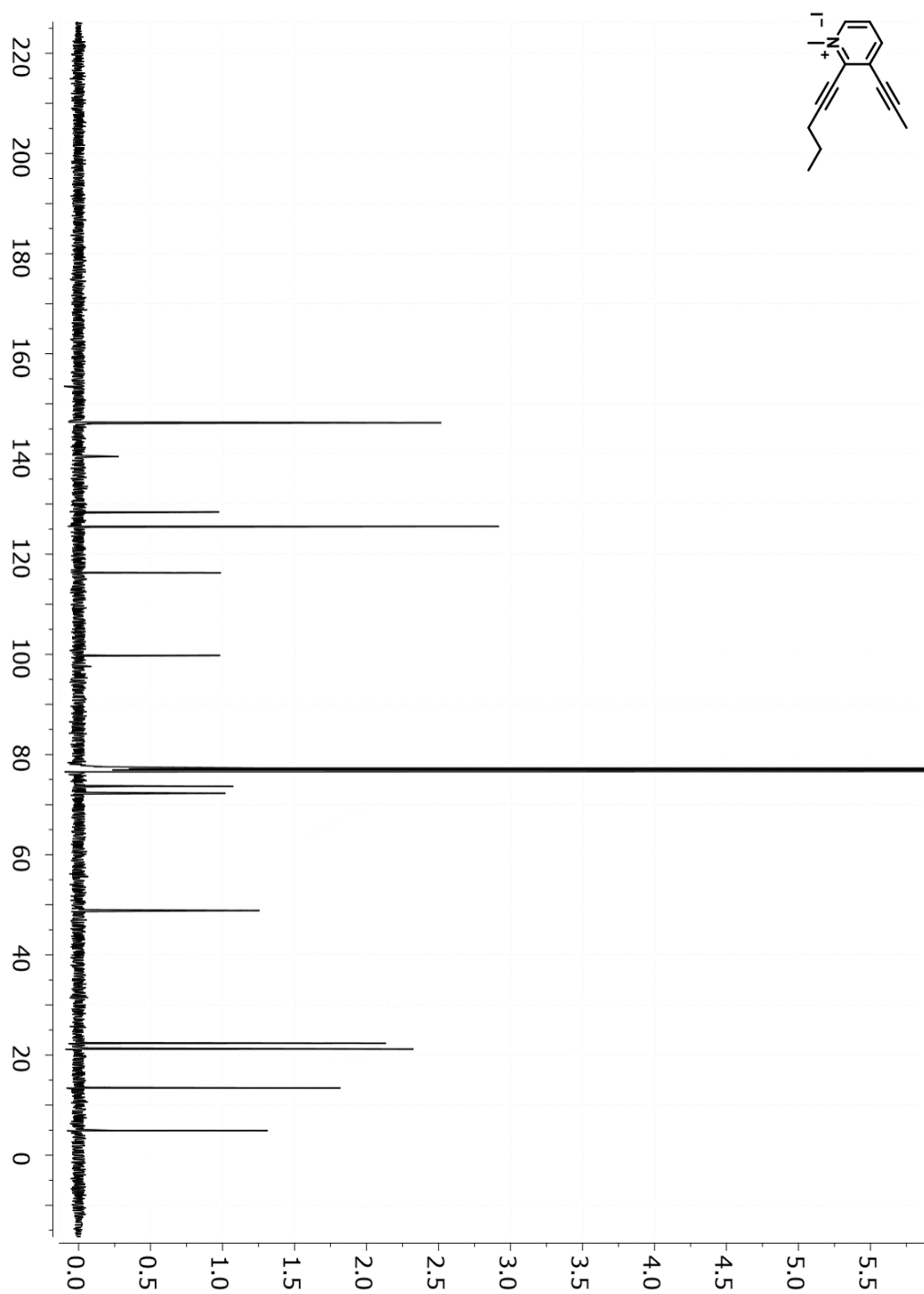
Figure 3.19. ^{13}\text{C}\{^1\text{H}\} NMR spectrum of 52 ( \text{CDCl}_3 , 100 MHz).
