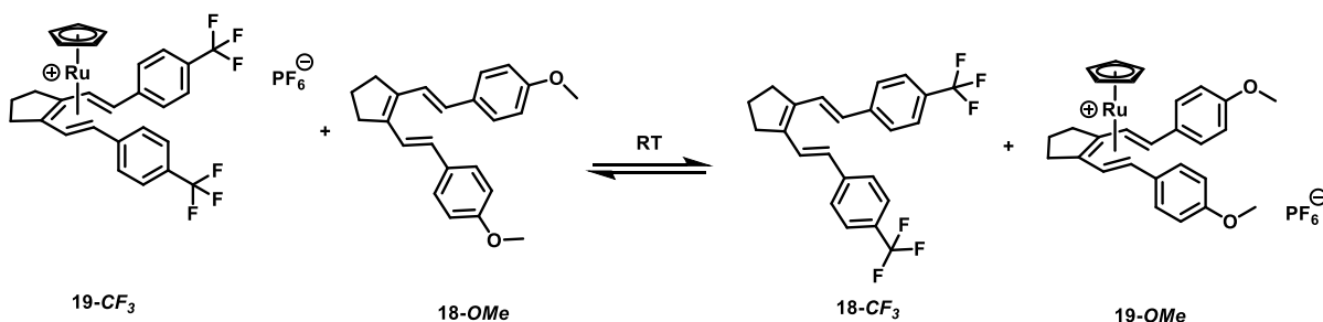
Scheme 2.9. Equilibrium experiment with 19-CF 3 and 18-OMe .
