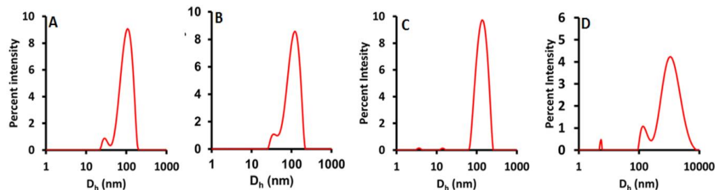
Figure 4.9. DLS of polymer 4b (A) Before UV irradiation pH 7.4 in 0.02M MOPS buffer (B) After UV irradiation 3 min pH 7.4 in 0.02M MOPS buffer (C) Before UV irradiation pH 5.5 in 0.02M MES buffer and (D) After UV irradiation 3 min pH 5.5 in 0.02M MES buffer.
