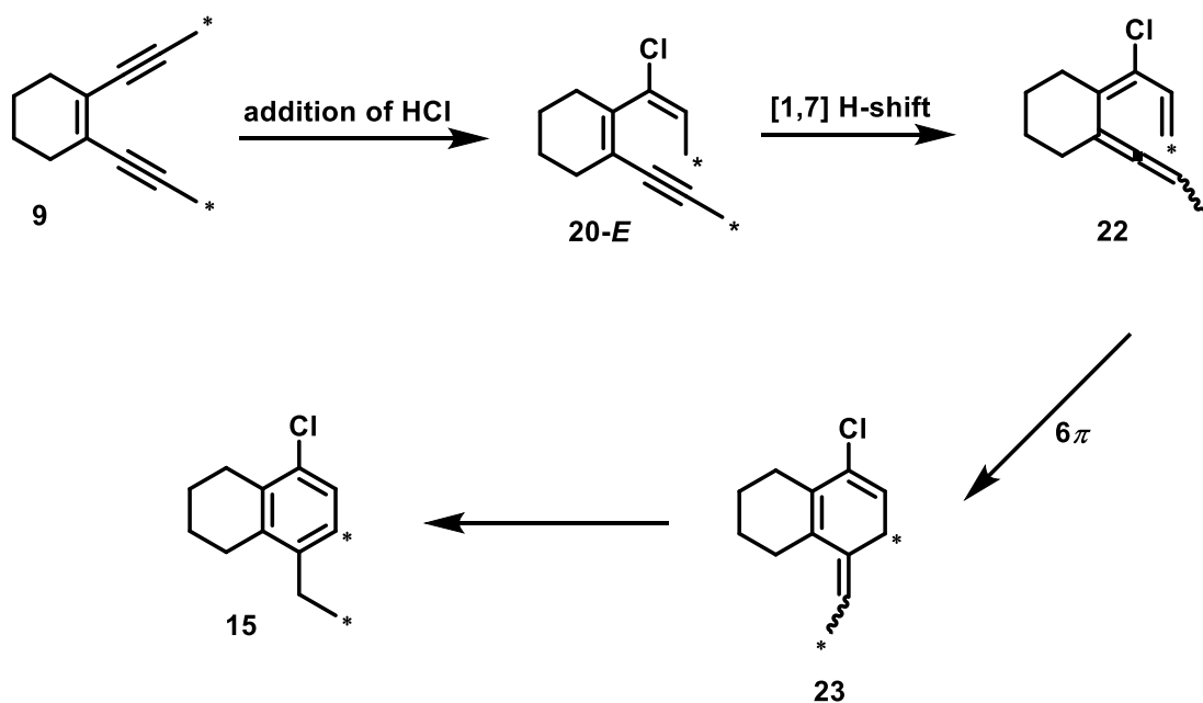
Scheme 3.5. Mechanistic hypothesis of the conversion of 9 to 15 . 4
