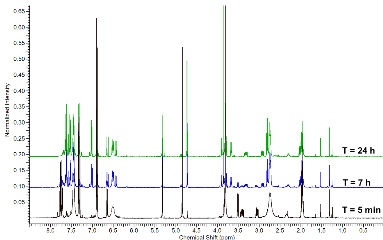
Figure 2.12. Equilibrium experiment with 19-CF 3 and 18-OMe . Time points were taken at 5 min, 7 h and 24 h. Ratios were calculated via the integration of the vinyl ( ^1\text{H} NMR \text{DC}_2\text{Cl}_2 , 500 MHz).
