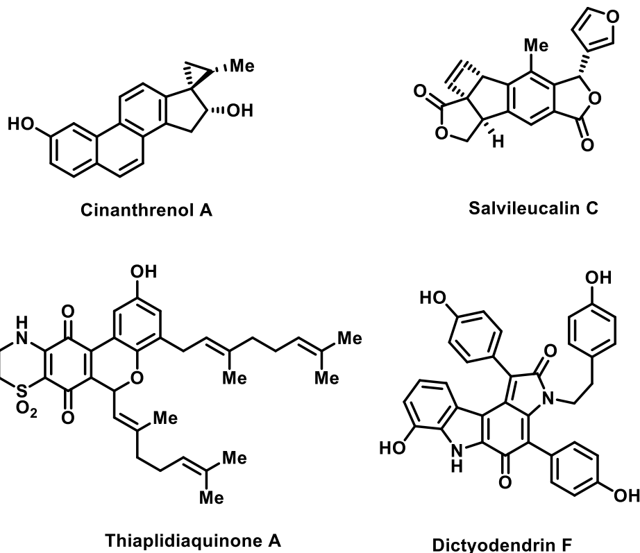
Figure 1.2. Selected examples of natural products synthesized via electrocyclization reactions. 2
