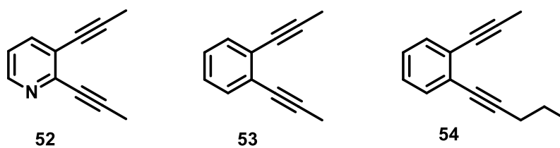
Figure 3.7. Enediyne molecules of future interest.
