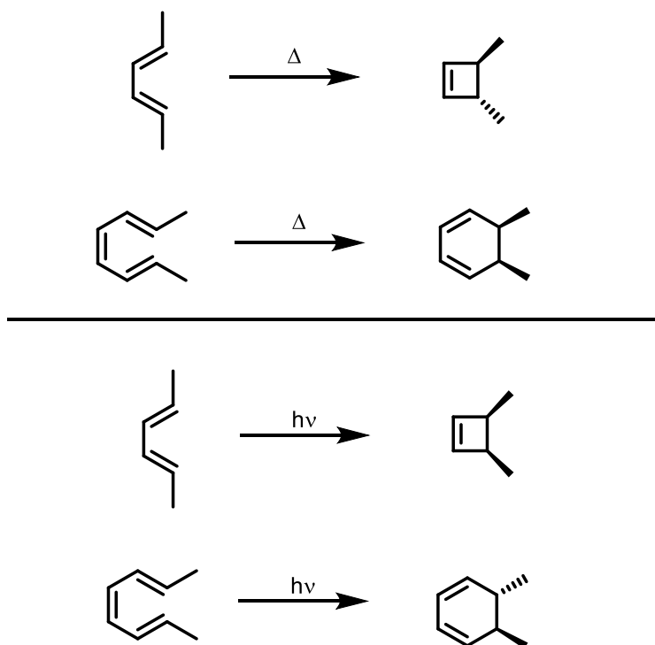
Scheme 1.1. Stereochemical electrocyclization outcomes under thermal (top) and photochemical (bottom) conditions as predicted by orbital symmetry conservation.
