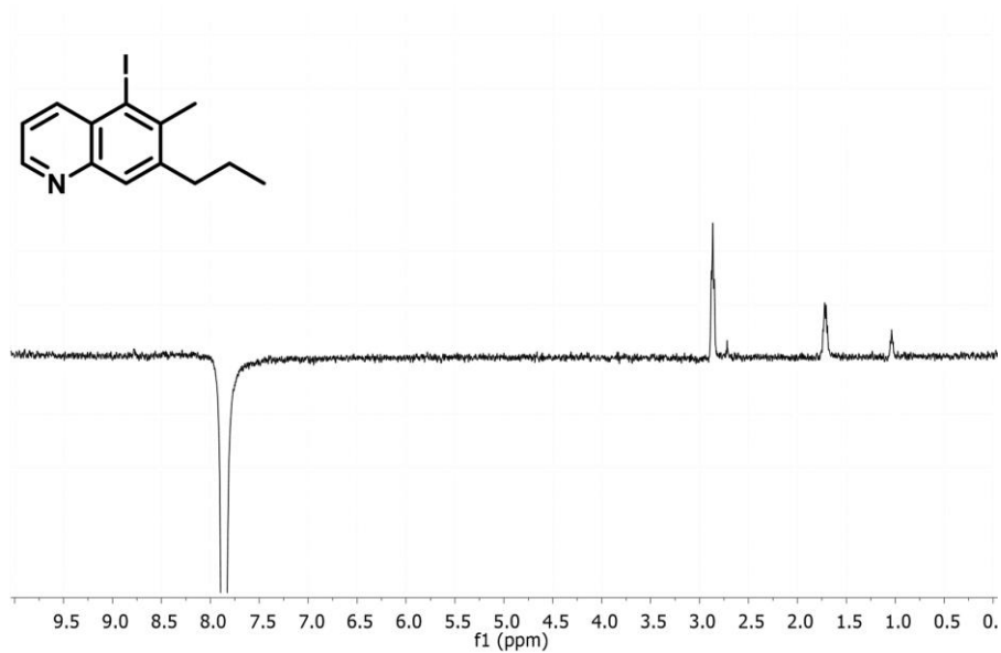
Figure 3.6 NOE spectrum of 29-I (500 MHz, \text{CDCl}_3 ).
