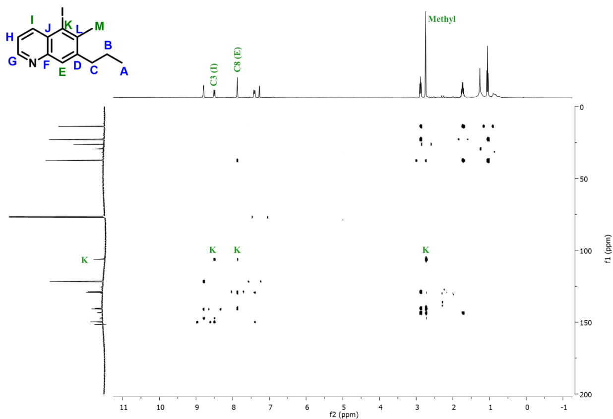
Figure 3.5. HMBC spectrum of 29-I (500 MHz, \text{CDCl}_3 ).
