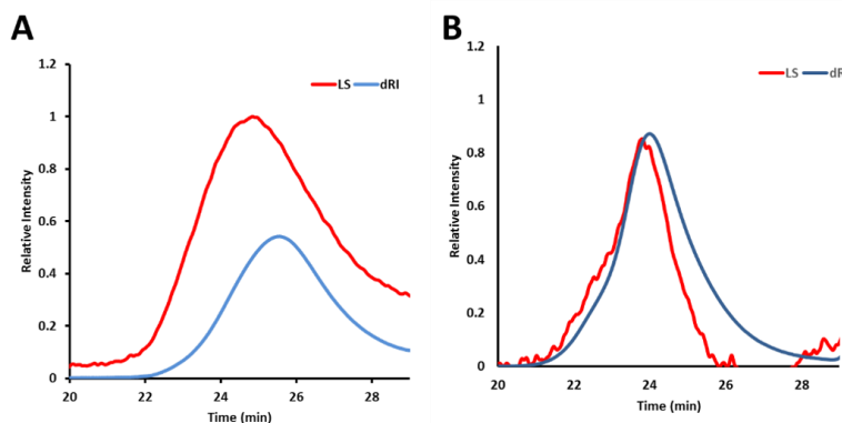
Figure 4.4. SEC-MALS traces of cross-linking control reaction. (A) SEC-MALS traces of polymer 2 in DMF as the eluent M_n = 44,000 \bar{D} = 1.1 and (B) after loading 2 nd generation Grubbs' and utilizing ethyl vinyl ether as a cross metathesis reactant. DMF as the eluent M_n = 46,000 \bar{D} = 1.1 . There is no evidence of crosslinked polymers based on SEC-MALS.
