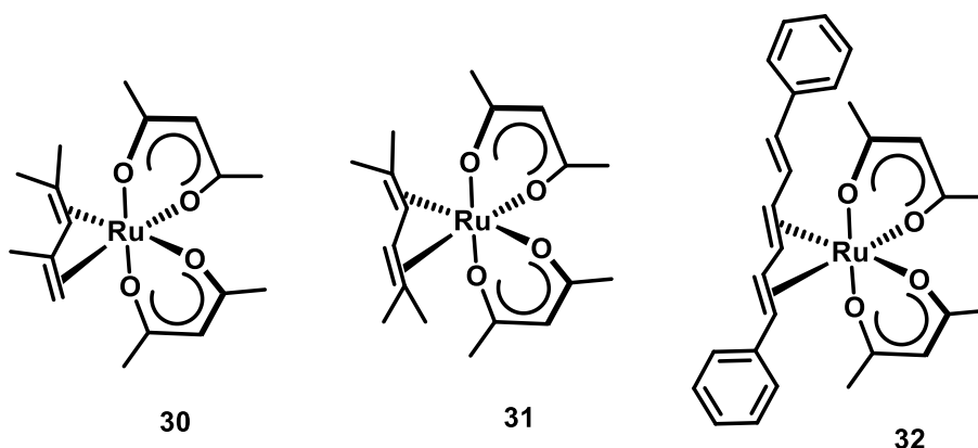
Figure 2.10. Known \text{Ru}(\eta^4\text{-trans-diene}) complexes.
