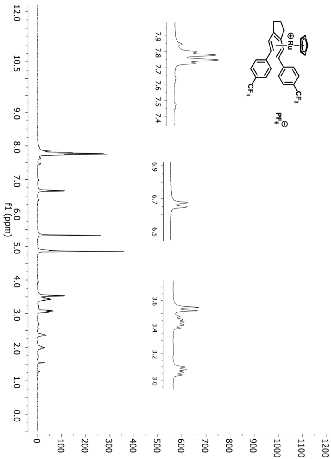
Figure 2.20. ^1\text{H} NMR spectrum of 19 -CF 3 (CD 2 Cl 2 , 400 MHz).
