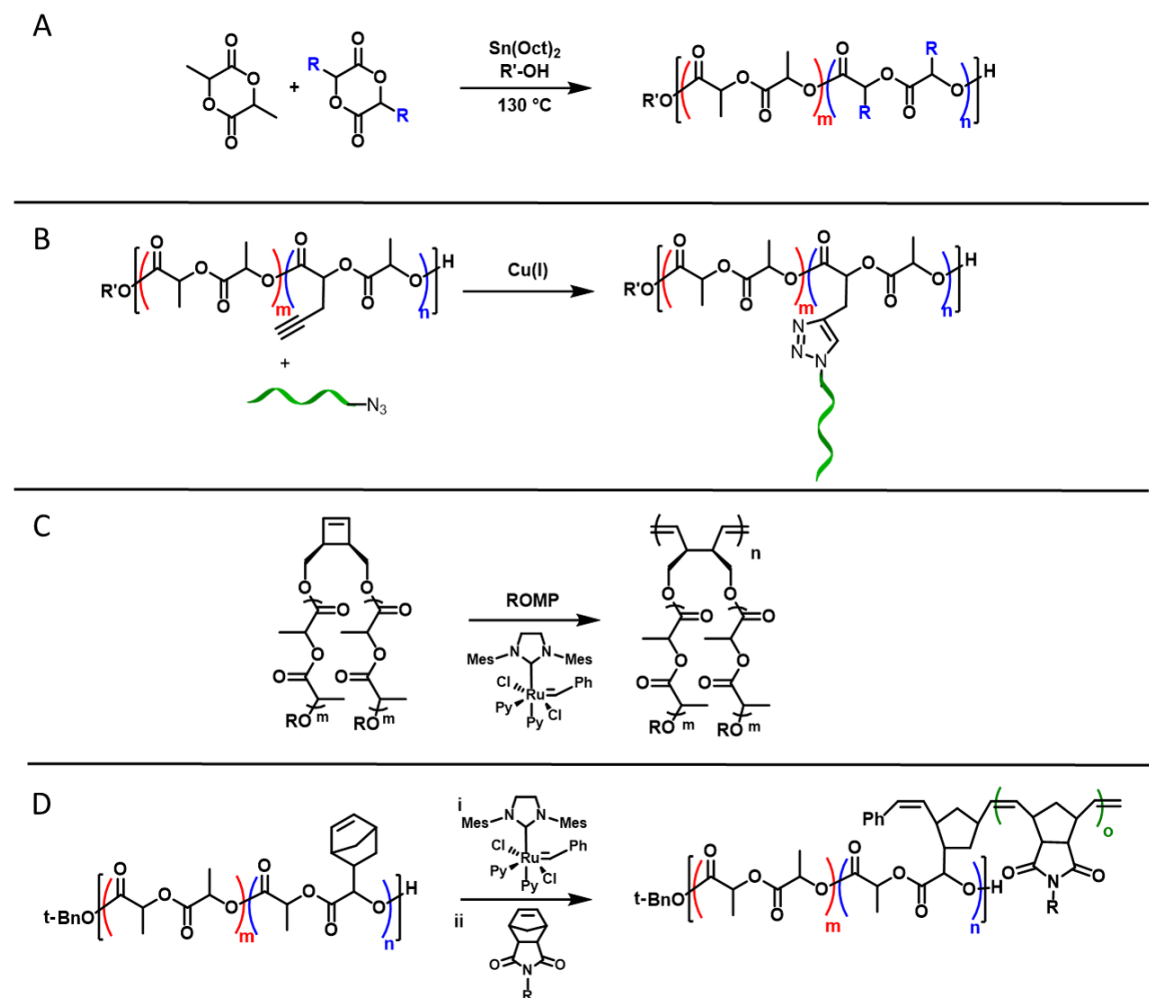
Figure 4.1. Strategies for the functionalization of PLA. (A) Copolymerizing R-functionalized lactide (B) graft-to polymerization. (C) graft-through polymerization. (D) graft-from polymerization (this work).
