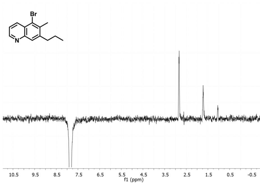
Figure 3.4 NOE spectrum of 29-Br (500 MHz, \text{CDCl}_3 ).
