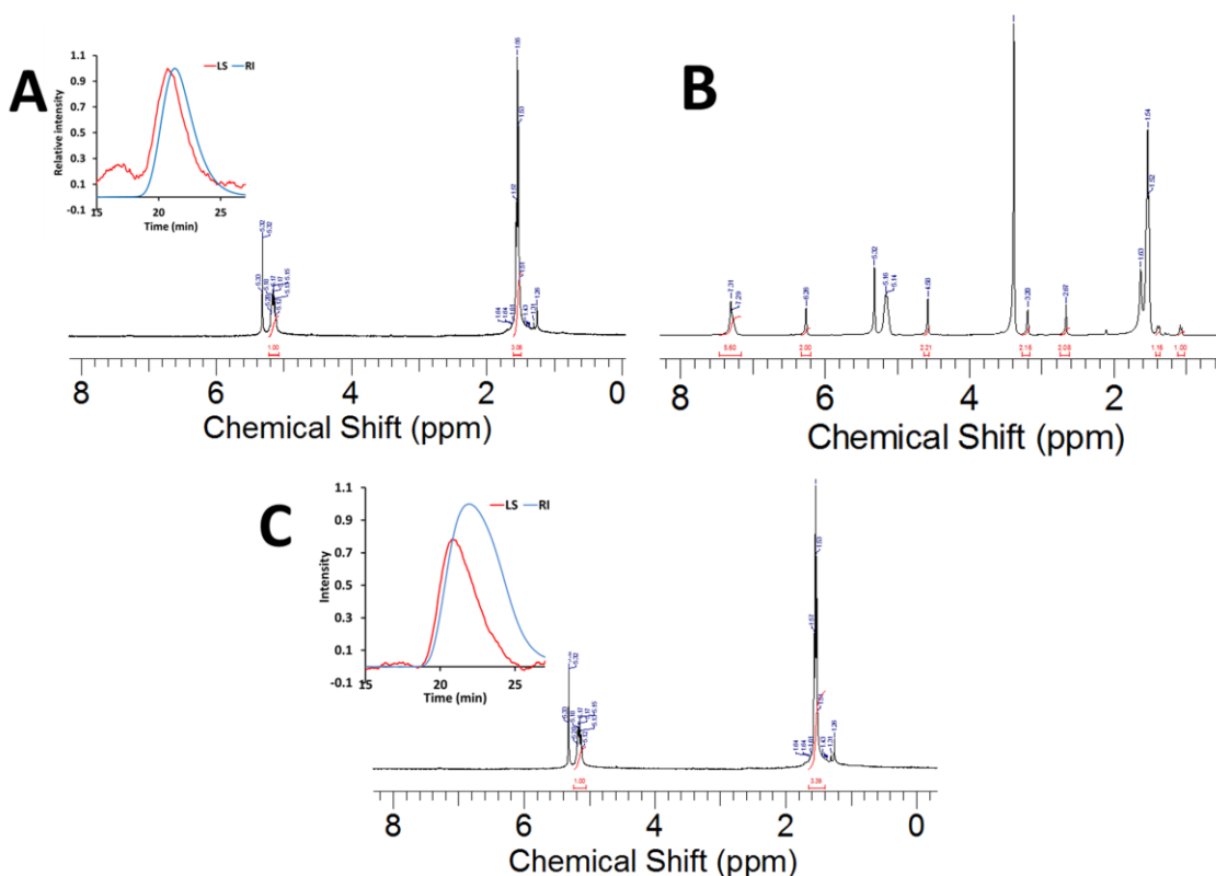
Figure 4.3. (A) Before reaction SEC-MALS in DMF as the eluent ( M_n = 12,000 and \text{Đ} = 1.2 ) and ^1\text{H} NMR. Unfunctionalized PLA polymer was added to a solution of 2 nd generation Grubb's catalyst followed by precipitate with cold degassed methanol (B) Add 5 equivalents of phenyl monomer ^1\text{H} NMR t = 30 min. None of the phenyl peaks in the NMR are broadened and olefin peak \delta = 6.26 ppm is still present which indicates no polymerization. (C) After the reaction: SEC-MALS in DMF as the eluent ( M_n = 13,000 and \text{Đ} = 1.3 ) and ^1\text{H} NMR. The product was precipitated with cold MeOH which yielded unfunctionalized PLA.
