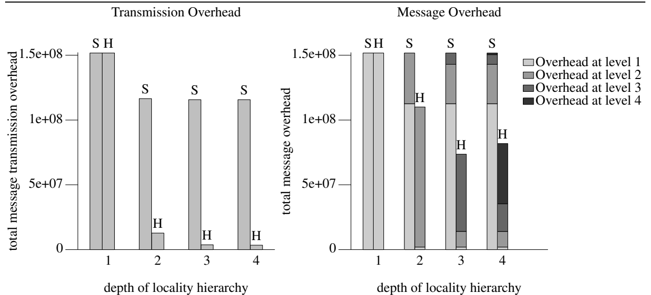
Figure 2 The performance of HCML compared with SCML in terms of both total message overhead and total transmission overhead.
