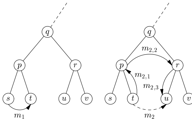
Figure 1 An example of a simple run with HCML.
