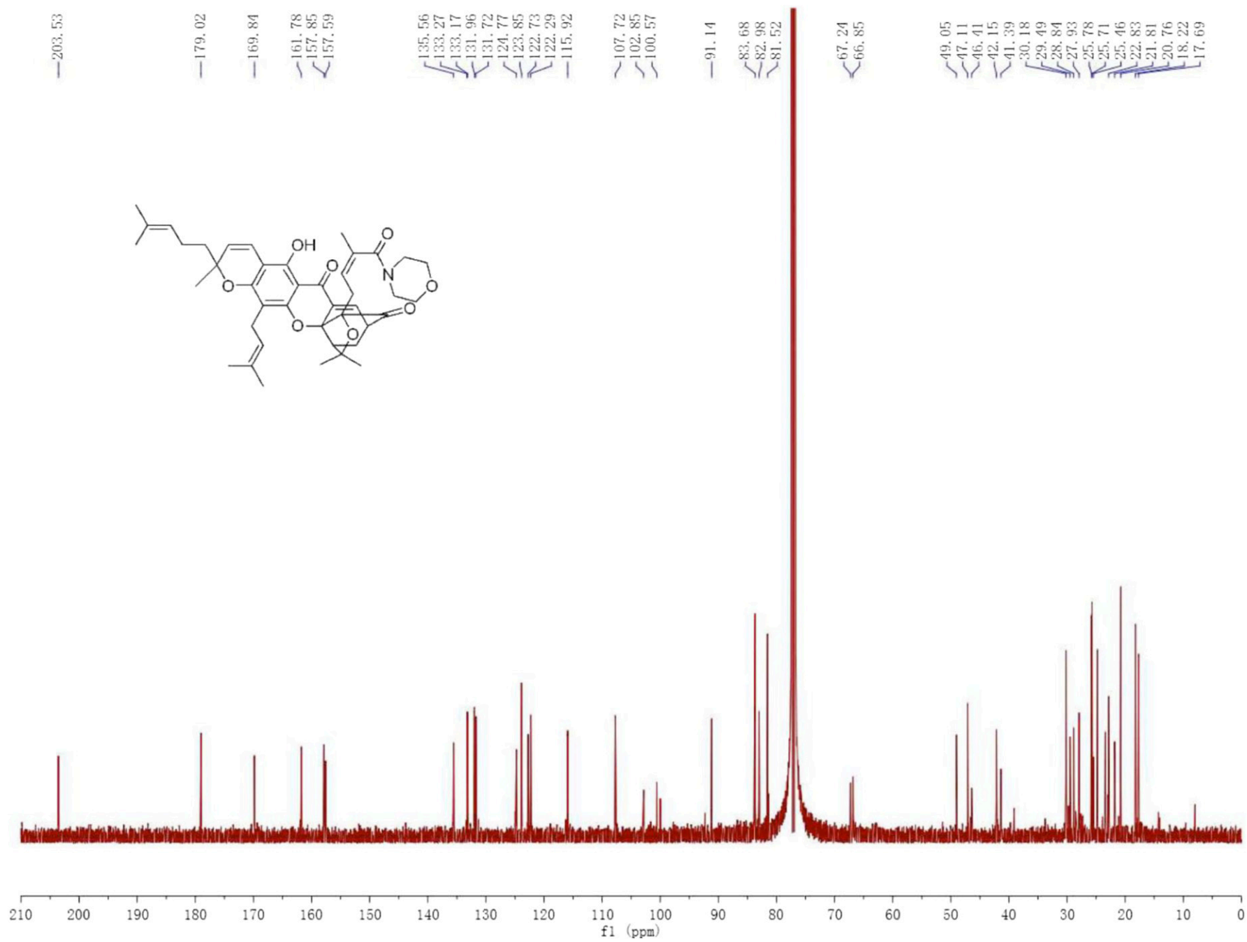
Fig. S7. ^{13}\text{C} NMR spectrum of DAP-19.
