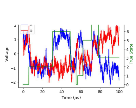
Example of filtered qubit parity traces (Credit: UC Berkeley)
