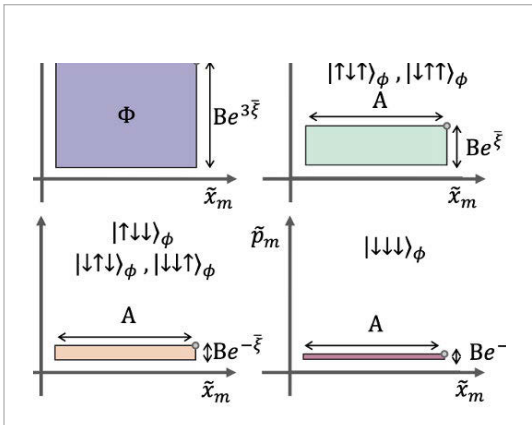
Protocols for entangling three ions (Credit: Duke University)
