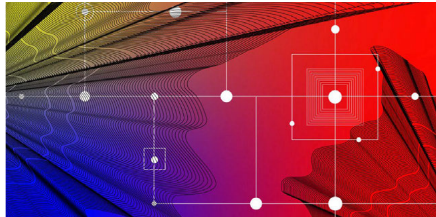
Researchers executed several quantum circuits on different physical platforms to analyze cross-platform fidelities (Credit: U Maryland)
