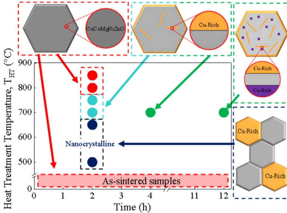
Figure 6. T_{HT} vs hold time demonstrating the effect of heat-treatment conditions on the electronic structure. Closed circles correspond to samples measured using XA spectroscopy, with the color corresponding to the phase and electronic states from Figure 5. Arrows connect microstructure and phase morphology schematics, derived from Figure 3 and our previous work [7], to their relevant heat-treatment conditions. The color coding designates the proposed thermodynamic driver for the observed phase and electronic structure state. Red corresponds to states that are driven by entropy. Green and light blue correspond to states in the coarse-grained samples that are influenced by enthalpy. Dark blue corresponds to states in the nanocrystalline samples that are influenced by enthalpy.
