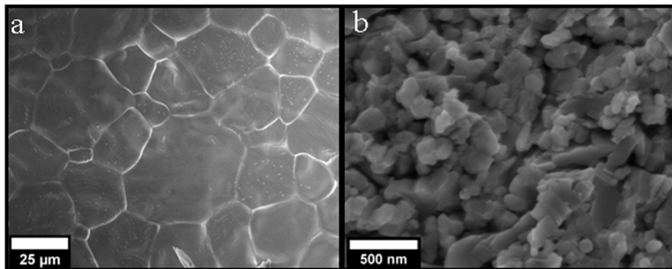
Figure 1. Microstructures of the consolidated (Co,Cu,Mg,Ni,Zn)O samples. (a-b) Fracture surface micrographs of the (a) 1100 °C conventionally sintered, single-phase coarse-grained sample (CG-AS), and (b) 700 °C SPS consolidated, single-phase nanocrystalline sample (NC-AS).
