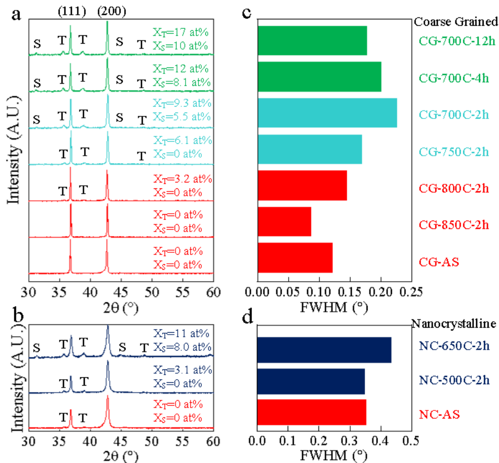
Figure 2. Interrogation into the phase state and lattice distortion. (a-b) XRD patterns for the (a) coarse-grained and (b) nanocrystalline samples after heat treatment at the designated T_{HT} and
