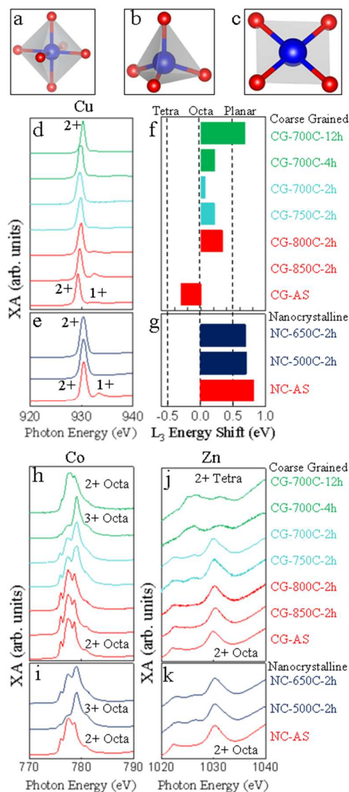
Figure 4. Role of heat treatment and grain size on the electronic structure (valence state and cation coordination). (a-c) Example schematics of element-independent cation coordination states: (a) octahedral, (b) tetrahedral, and (c) planar. (d-e) Cu L_3 spectra for the (d) coarse-grained and (e) nanocrystalline samples after various heat treatments. (f-g) The peak energy shift (in eV) of the \text{Cu}^{2+} L_3 peak, relative to the T_{HT} = 850^\circ\text{C} 2 h, single-phase sample (CG-850C-2h), for the (f) coarse-grained and (g) nanocrystalline samples after various heat treatments. Dashed
