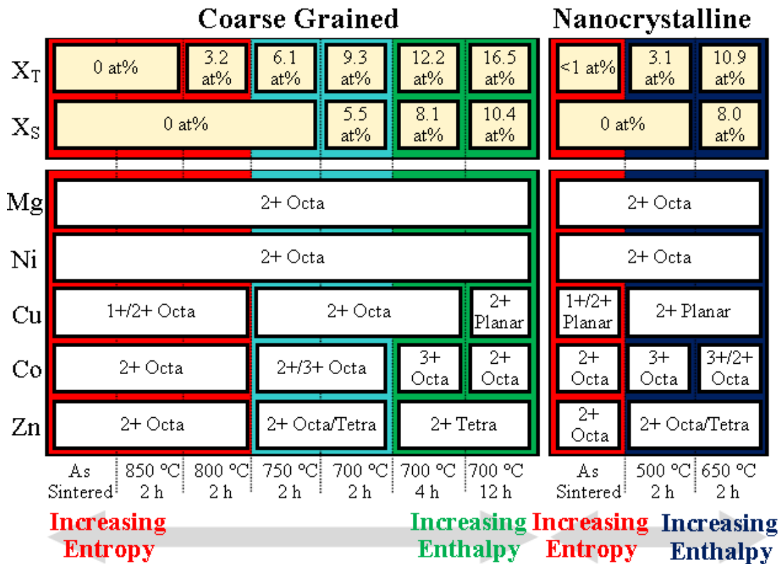
Figure 5. Evolution of the electronic structure (valence state and cation coordination). Table summarizing the evolution in tenorite ( X_T ) and spinel ( X_S ) secondary phases as well as the evolution in electronic structure for all five cations. The corresponding heat-treatment conditions are listed at the bottom of each column. The color coding designates the proposed thermodynamic driver for the observed phase and electronic structure state. Red corresponds to electronic structure states that are driven by entropy. Green and light blue correspond to electronic structure states in the coarse-grained samples that are influenced by enthalpy. Dark blue corresponds to electronic structure states in the nanocrystalline samples that are influenced by enthalpy.
