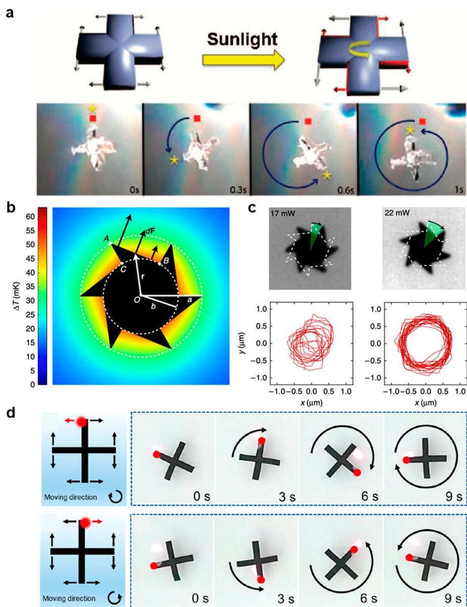
Figure 28. Optothermal Marangoni rotors. (a) Schematic and optical images showing the rotation of a cross-shaped Marangoni rotor with light-absorbing material embedded on the clockwise face of each fin. Adapted with permission from ref 377. Copyright 2009 American Chemical Society. (b) Simulation of the temperature distribution at the light-irradiated rotor. A, B, and C represent different intersection points, respectively, while a and b are the outer and inner radii of the rotor, respectively. (c) Trajectories of the rotational rotor driven by laser beams with different powers. Adapted with permission from ref 256. Copyright 2015 Springer Nature. (d) Clockwise (top) and counterclockwise (bottom) rotation of the cross-shaped rotor at the liquid–air interface. Adapted with permission from ref 380. Copyright 2020 American Chemical Society.
