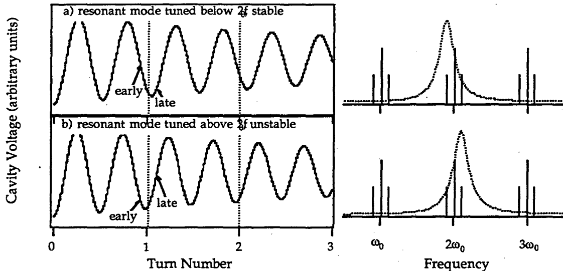
Fig. 12.15. A time-domain view of a resonator voltage driving a longitudinal coupled-bunch instability and the corresponding frequency domain view. The sidebands of the revolution harmonics represent the phase modulation of the beam current resulting from the synchrotron oscillations, and the dashed line is the resistive part of a resonator impedance.
