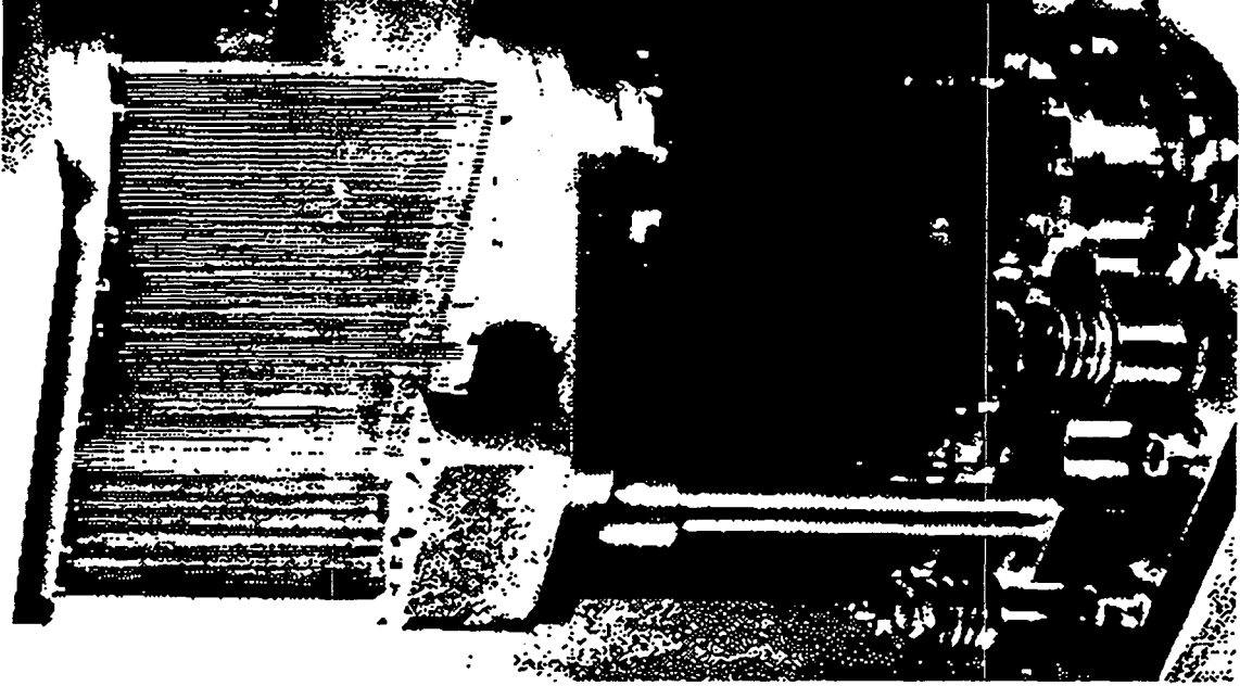
Fig. 12.2. A transition joint in the vacuum chamber in the injection region of the ALS. The joint must be flexible in order to accommodate a transverse motion of a few cm during injection. The required flexibility and low impedance is achieved by a "wire cage" design (the entire assembly shown is enclosed in a large bellows in order to maintain the vacuum). If the joint had been left open, the discontinuity would have led to a large impedance. Photo courtesy of J. Corlett.
