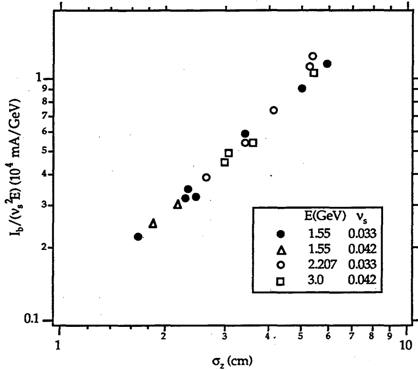
Fig. 12.8. Turbulent bunch lengthening measured at SPEAR.
