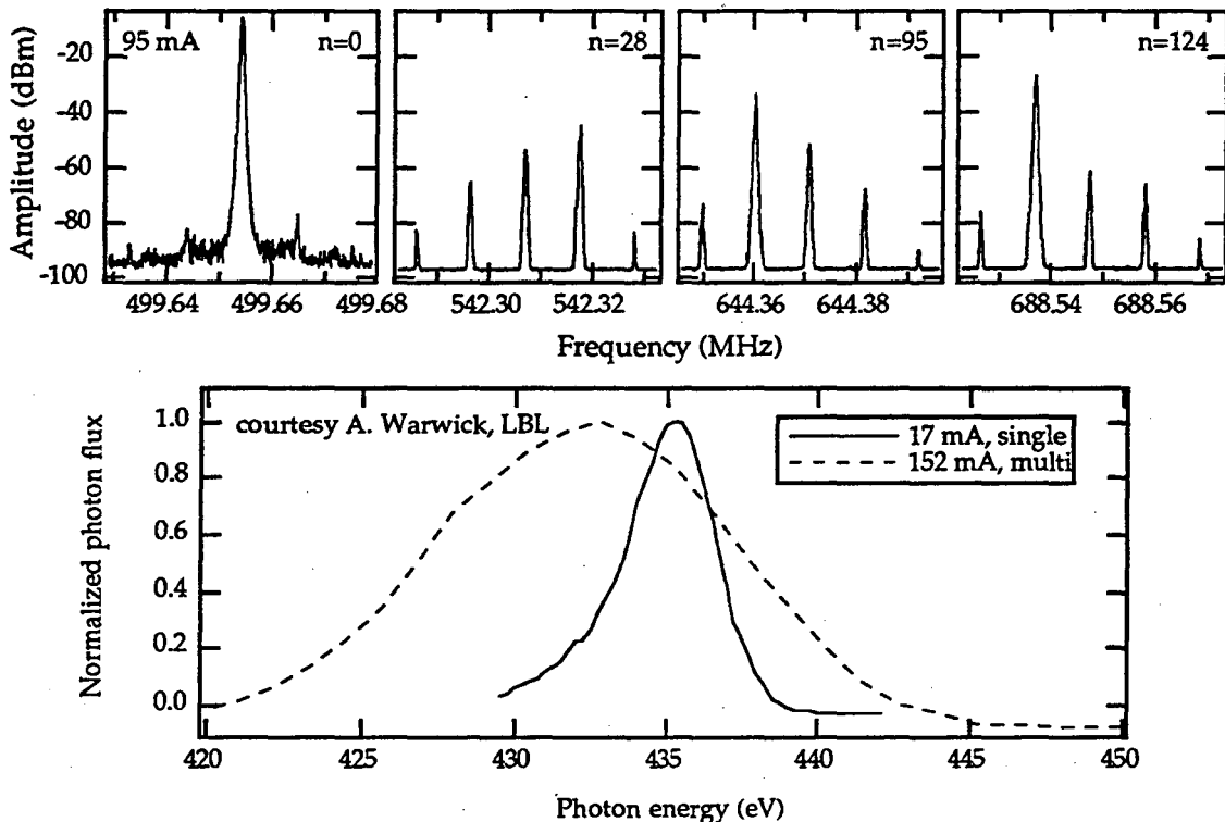
Fig. 12.16. The ALS electron beam spectrum near several revolution harmonics with all RF buckets filled indicates large amplitude longitudinal coupled-bunch oscillations. The central peak in each graph is the signal at the n th revolution harmonic above the RF frequency and the phase modulation sidebands are oscillations of various normal modes of the beam. The bottom graph shows initial measurements of the undulator 3rd harmonic taken under similar conditions during the commissioning of an ALS undulator. A marked increase in the spectral width of higher harmonics of the synchrotron light results from the coupled-bunch energy oscillations.
