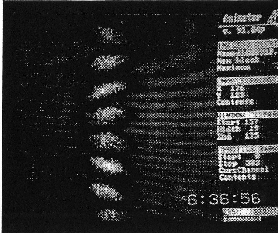
Fig. 12.10. Turn-by-turn pictures of a bunch executing vertical head-tail oscillations in the electron storage ring LEP. The bunch is observed from the side. The synchrotron tune is \sim 0.1 . The horizontal scale is 1000 ps for the total image, not counting the table of numbers at the right. The vertical scale is uncalibrated, but the vertical rms beam size is \sim 0.2 mm at the observation point. Photo courtesy of E. Rossa.
