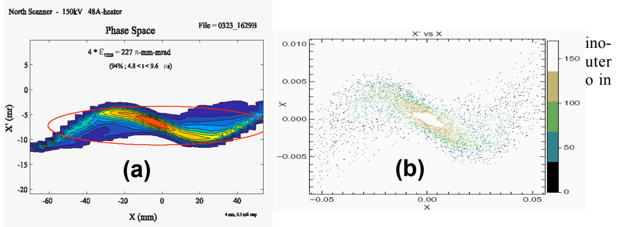
Figure 2 (a) Experimental phase space measured for an unapertured beam created with a 10-cm diameter alumino-silicate surface ionization source. (b) Warp-3-D particle-in-cell simulation of the experiment depicted in (a).
