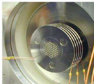
Figure 1: Source Test Stand (STS-100): Sixty-one beamlets have been extracted from an RF-argon plasma source, through a grid supported by three multi-layer high gradient insulator stacks (not visible), with brightness and uniformity meeting requirements for heavy ion fusion.
