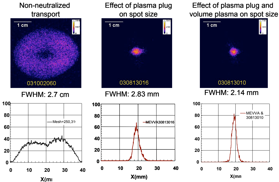
Figure 4. The Neutralized Transport Experiment (NTX) showing beam images at the focal plane for three cases of space-charge neutralization for a high perveance ( 6 \times 10^{-4} ), 25 mA, 300 keV K^+ ion beam: left: no preformed plasma; center: localized “plug” plasma just beyond the last focusing magnet, and right: with both “plug” and “volume” preformed plasma.
