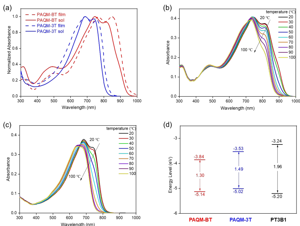
Figure 2. a) Normalized UV-vis absorption spectra of PAQM-BT and PAQM-3T in chlorobenzene and thin film at room temperature. The evolution of UV-vis absorption spectra of b) PAQM-BT and c) PAQM-3T in chlorobenzene when heated from 20 °C to 100 °C. d) Diagram of energy levels and bandgaps of PAQM-BT, PAQM-3T and PT3B1.
