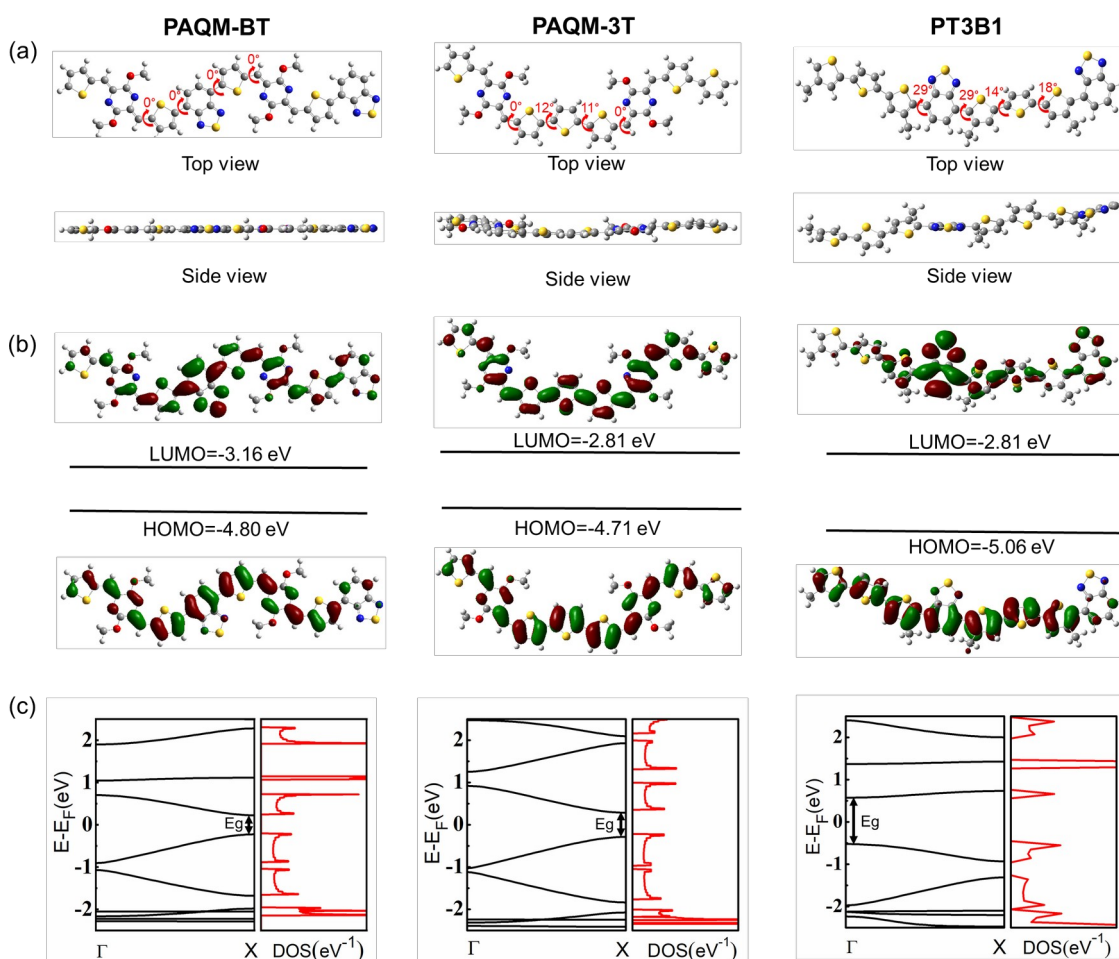
Figure 5. a) Optimized geometries of the dimeric segments of the three polymers, in which alkyl chains are substituted with methyl groups to simplify the calculation. b) Calculated molecular orbital distribution and energy levels of the dimeric segments of three polymers. c) Band structures and partial densities of states (DOS) of three polymers.
