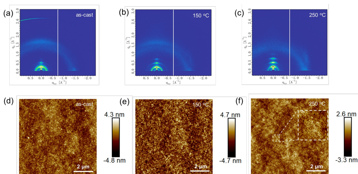
Figure 4. GIWAXS patterns of PAQM-BT of a) as-cast film, b) 150 °C annealed film and c) 250 °C annealed film. AFM images of PAQM-BT of d) as-cast film, e) 150 °C annealed film and f) 250 °C annealed film.
