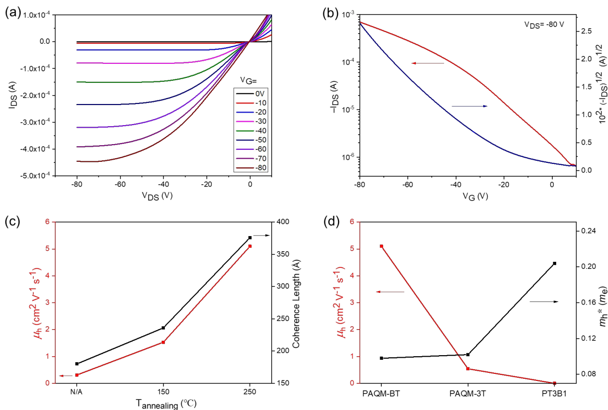
Figure 3. Typical a) output and b) transfer characteristics of OFETs based on PAQM-BT annealed at 250 ^{\circ}\text{C} . c) Hole mobilities and coherence length of PAQM-BT at different annealing temperature. d) Hole mobilities and effective hole masses of PAQM-BT, PAQM-3T and PT3B1.
