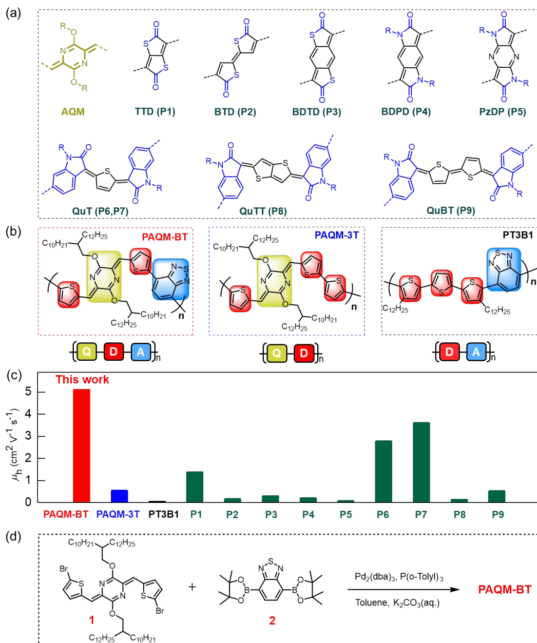
Figure 1. a) p -AQM and other typical ground-state quinoidal units. Related quinoidal-aromatic polymers from the literature are listed in parentheses with structures illustrated in Figure S1. b) Molecular structures of PAQM-BT reported in this work and reference polymer PAQM-3T and PT3B1. c) A comparison of hole mobilities of PAQM-BT, PAQM-3T, PT3B1 and other
