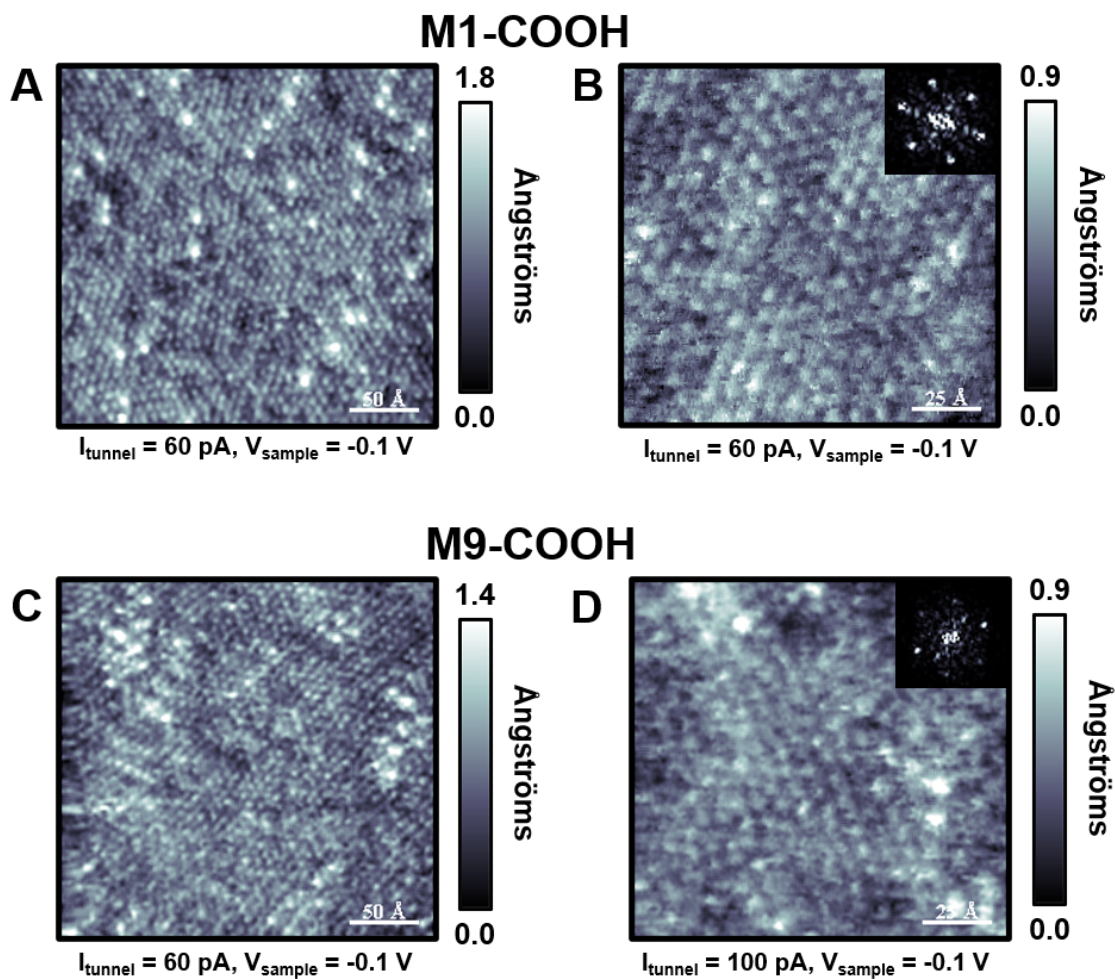
Figure 2. Scanning tunneling microscopy images of (A,B) M1-COOH and (C,D) M9-COOH self-assembled on Au{111}. All images were taken at ambient conditions. Insets depicting Fourier transforms of (B) and (D) show hexagonal close-packed arrays with identical nearest-neighbor distances of 8.4 \pm 0.4 \text{ \AA} for both isomers.
