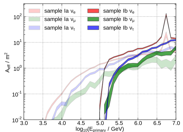
FIG. 10. Effective areas for different neutrino flavors in samples Ia and Ib.
