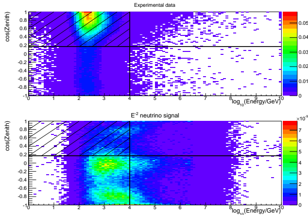
(a) The IceCube-40 Level 3 zenith angle and energy reconstructions. The two panels show the data and E^{-2} spectrum electron neutrino signal. The Level 3 cuts are represented by the black lines at zenith \Theta_{\text{track}} = 80^\circ and energy E_{\text{ACER}} = 10 \text{ TeV} . Events in the hatched upper left quadrant of each of the panels were removed.
