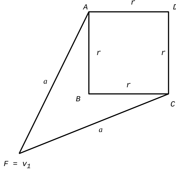
Figure 10: The Peaucellier invensor.
