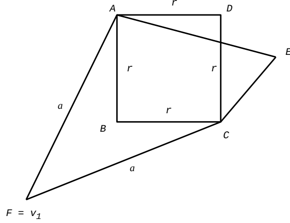
Figure 11: The modified Peaucellier inversor \mathcal{J}_t : the square ABCD is rigidified and \ell[AE] - \ell[EC] = 2\epsilon > 0 , \ell[EC] > r .
