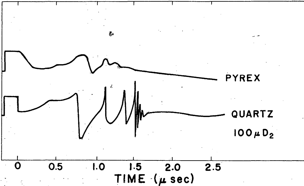
VOLTAGE ACROSS A PINCH IN PYREX AND QUARTZ INSULATOR TUBES
