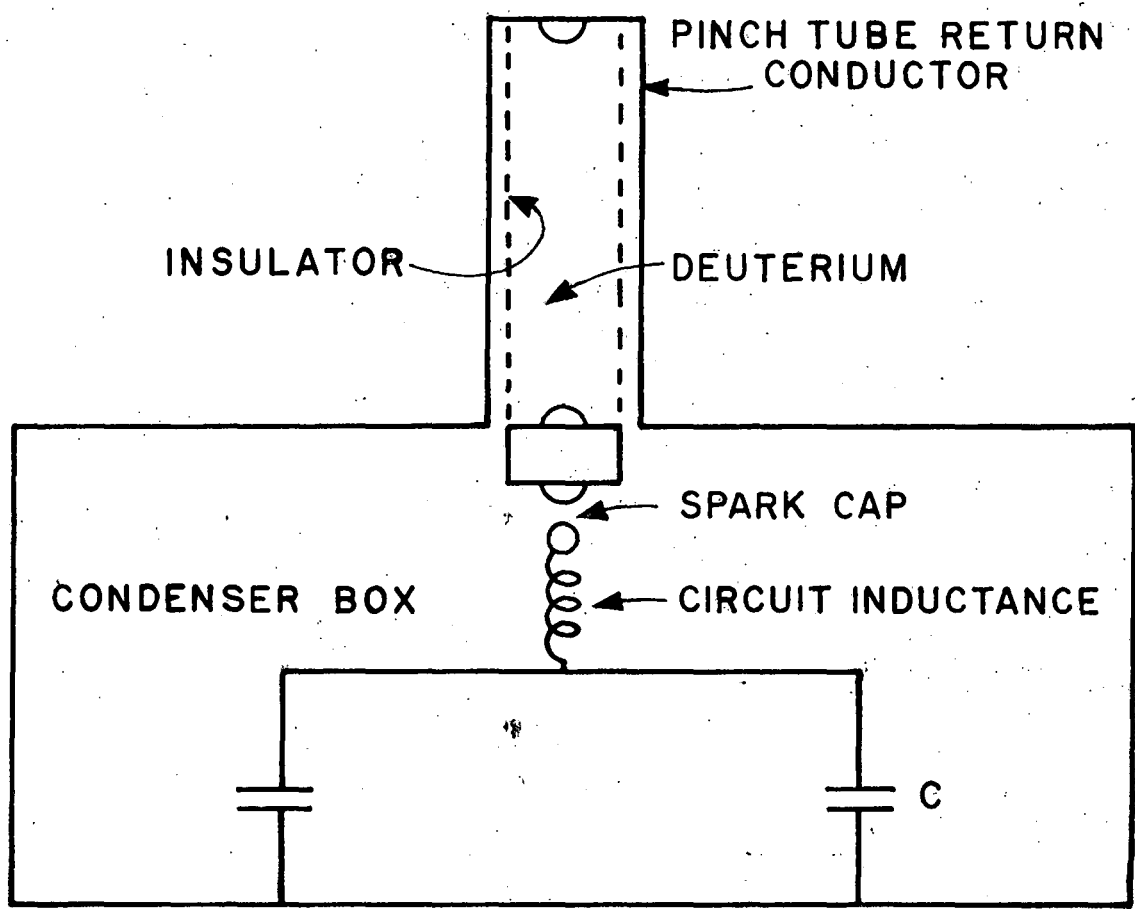
PINCH CIRCUIT SCHEMATIC
