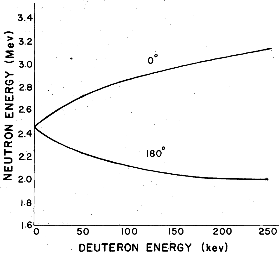
NEUTRON ENERGIES FROM D-D REACTIONS AS A FUNCTION OF INCIDENT DEUTERON ENERGY
