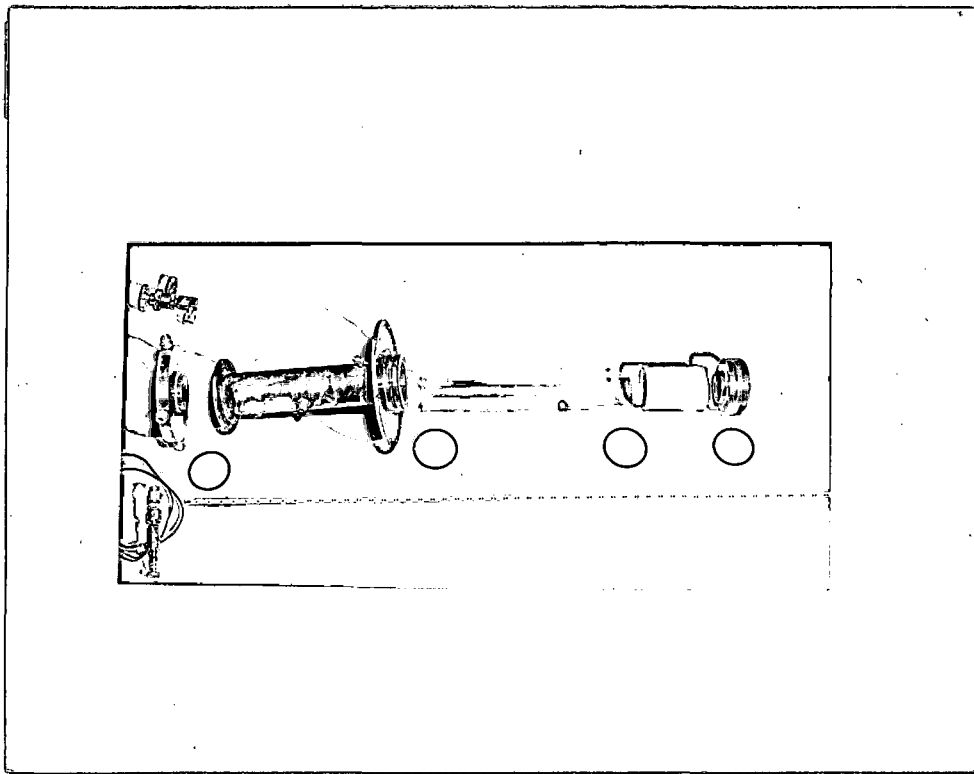
Fig. 3. Exploded view of a pinch tube.
