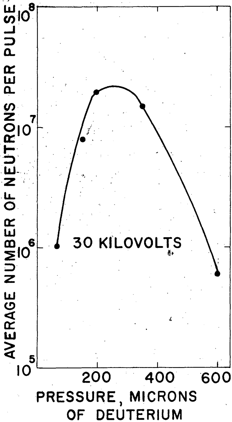
NEUTRON YIELDS VS. VOLTAGE AND PRESSURE IN 5 cm X 45 cm QUARTZ TUBE
