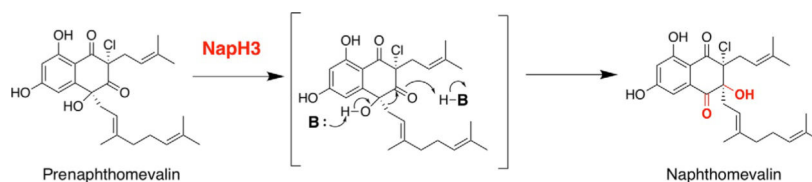
Fig. 5. NapH3 α-hydroxyketone rearrangement of synthetic “prenaphthomevalin” to generate naphthomevalin (B: represents a general base in the reaction).
