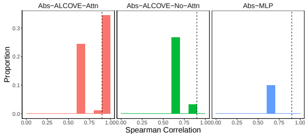
Figure 4: Histogram of correlation scores for the abstract simulations. Each panel shows the histogram of correlation scores for each of the abstract models. The vertical dashed line indicates the threshold for a correlation to represent a successful type ordering, and thus bars to the right of this line represent the set of simulations that produced correct type orderings.
