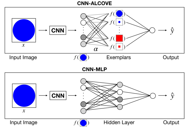
Figure 2: Architecture for the two categorization models. In both models, the image stimulus x is first passed through a pre-trained CNN, which extracts a high-level feature representation. For the CNN-ALCOVE model (top), this high-level representation is then reweighted based on the learnable attention parameters and its similarity computed to all of the other exemplars, then passed into a feedforward layer to predict its category label. For the CNN-MLP model (bottom), the extracted features are passed into a simple two-layer neural network which computes the category label without any attention or exemplar comparisons.
