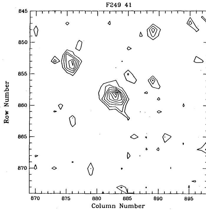
Fig. 15 Contour plot of the variable object identified as a galaxy by Jorge Melnick of the European Southern Observatory, using the NTT.
