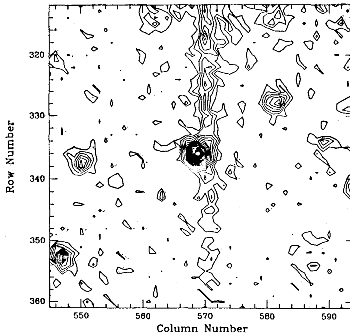
Fig. 15 Contour plot of the variable object identified as a galaxy by Jorge Melnick of the European Southern Observatory, using the NTT.
