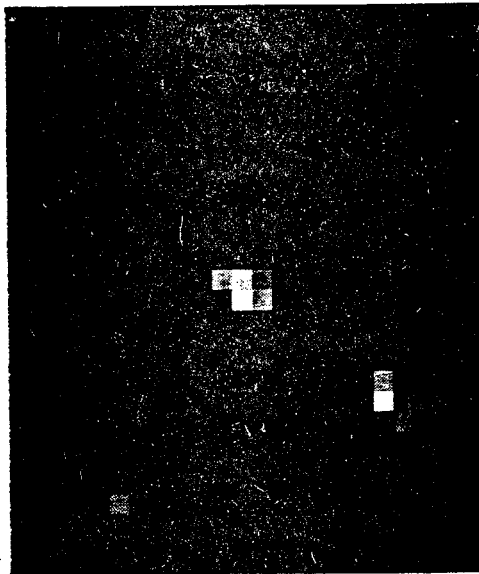
Fig. 14 The galaxy in F249-41 which has changed in magnitude and appears to have changed in shape as well.
