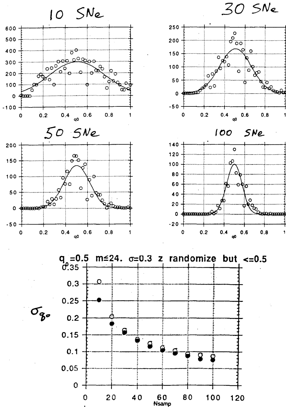
Fig.2 Monte Carlo distribution of "measured" q_0 = \Omega/2 for Gaussian distribution ( \sigma = 0.3 ) of Type Ia maximum light. Calculations by S. Perlmutter, to be published.
