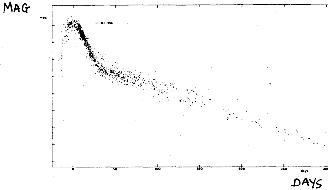
Fig.3 Composite blue light curve obtained by the fitting of the observations of 38 Type I supernovæ. One magnitude intervals are marked on the ordinates. Compilation by Barbon, Ciatti, and Rosino (1974).
