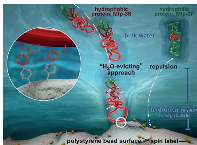
Figure 3. Mfp adsorption to surfaces requires the hydration layers to be broken through. Under force-free solution conditions, the strong hydration layers (gray-blue) surrounding Mfp-3F and the PS surface pose a double hydration barrier to adhesive interactions between these structures. In contrast, the weak hydration layers (light blue) of Mfp-3S facilitate the intimate approach of Mfp-3S to the PS surface by readily ejecting the initially surface bound hydration water molecules and subsequently mediating hydrophobic interactions as depicted in the magnified illustration in the circle.
