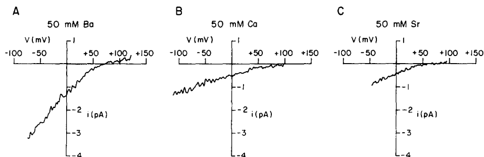
FIGURE 10. Comparison of single channel current-voltage relations with \text{Ba}^{2+} , \text{Ca}^{2+} , and \text{Sr}^{2+} . Methods as in Fig. 6. Pipette solutions as in Fig. 7C, with \text{CaCl}_2 and \text{SrCl}_2 substituting for \text{BaCl}_2 in B and C, respectively. Cells 26G, 25L, and 25S.
