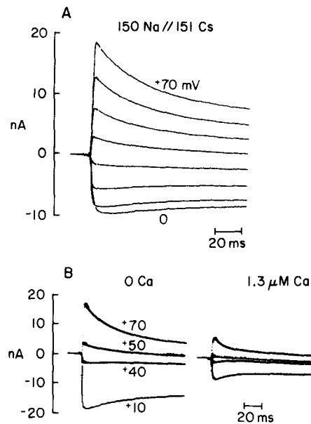
FIGURE 6. Ca channel selectivity for monovalent cations and sensitivity of monovalent currents to block by micromolar external Ca 2+ . (A) Superimposed traces of net current (linear leak and capacity currents subtracted). The external solution contained 150 mM NaCl, 5 mM Na-HEPES (pH 7.4), 2 mM Na 2 EGTA, and 12.5 μM TTX. The internal solution contained 151 mM CsCl 2 , 5 mM Cs-HEPES, and 10 mM Cs 2 EGTA. Cell 207B. (B) Same ionic conditions as in A. Net currents at four potentials in the absence (left, 2 mM Na 2 EGTA) and presence of micromolar external Ca 2+ (EGTA replaced by 10 mM HEDTA plus 5 mM Ca 2+ ; [Ca] 2+ = 1.3 μM at pH 7.4). Cell 207G.
