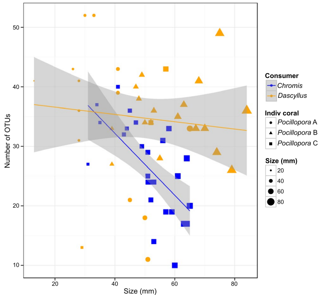
FIGURE 5 Diversity of OTUs in relation to fish size (total length in mm). A linear model is fitted with 95% confidence intervals. Chromis : Y = 53 - 0.5 * X , adjusted r^2 = 0.39 , p < 0.001 ; Dascyllus : Y = 37.8 - 0.1 * X , adjusted r^2 = 0.01 , p = 0.5 . The number of OTUs was calculated from the rarefied data set ( n = 259 ) to control for differences in sampling effort [Colour figure can be viewed at wileyonlinelibrary.com ]
