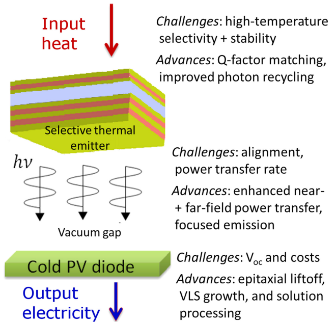
Figure 26. Overview of TPV operation along with a summary of the remaining challenges and possible advances to help address them.
