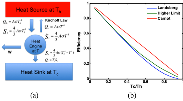
Figure 37. (a) A heat engine operating between a heat source at T_h and a heat sink T_c . Heat transfer between the engine and heat source is coupled via thermal radiation. Kirchoff's law dictates that some photons, their associated energy, and entropy are sent back to the heat source, (b) comparison of three different efficiencies, the Carnot, the Landsberg, and efficiency \eta_2 , which is higher than the Landsberg efficiency.
