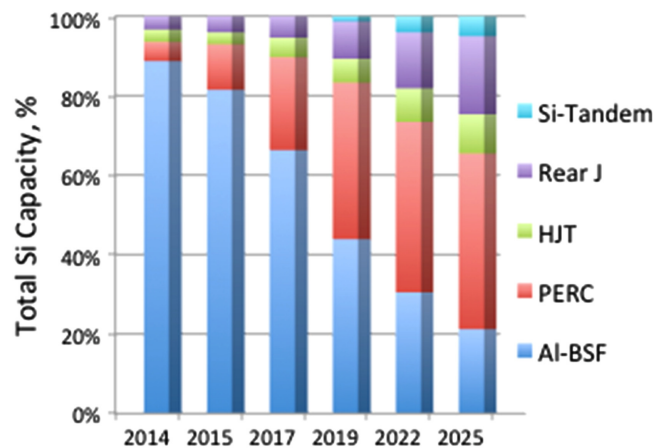
Figure 4. Industry consensus on the present and future market share of the different Si cell technologies of figure 3 (data extracted from [29]).
