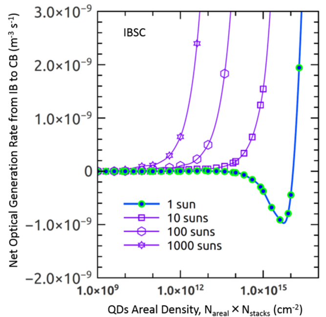
Figure 11. Detailed balance calculation of the dependence of G_{net} on concentration ratio. The IB is located at 0.2 eV below the CB edge. Reproduced with permission from [60].
